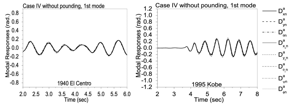
Figure 6. First-mode responses for El Centro earthquake in 1940 and Kobe earthquake in 1995 without pounding.
