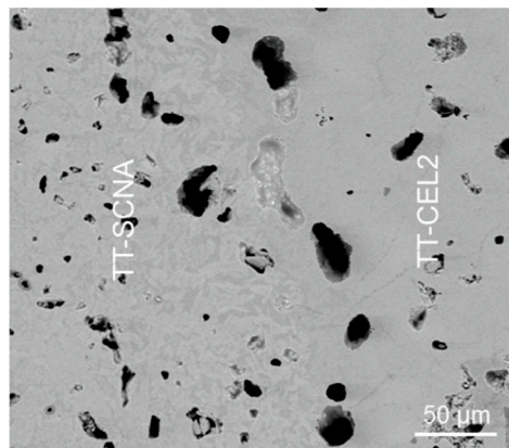
Figure 7. Bilayered glass-ceramic implant: interface between TT-CEL2 and TT-SCNA layers.
