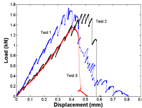
Figure 5. Experimental load vs. displacement curves for the three four-point bending tests conducted.
