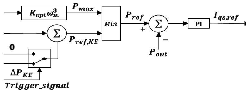
Figure 7. Modified q -axis rotational current control loop.
