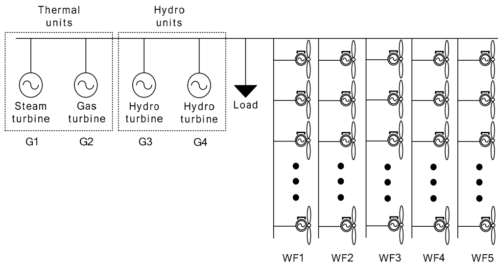
Figure 10. Simulated small power system.
