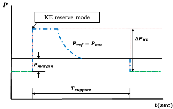
Figure 4. KE reserve control scheme.
