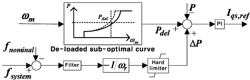
Figure 3. De-loaded controller.
