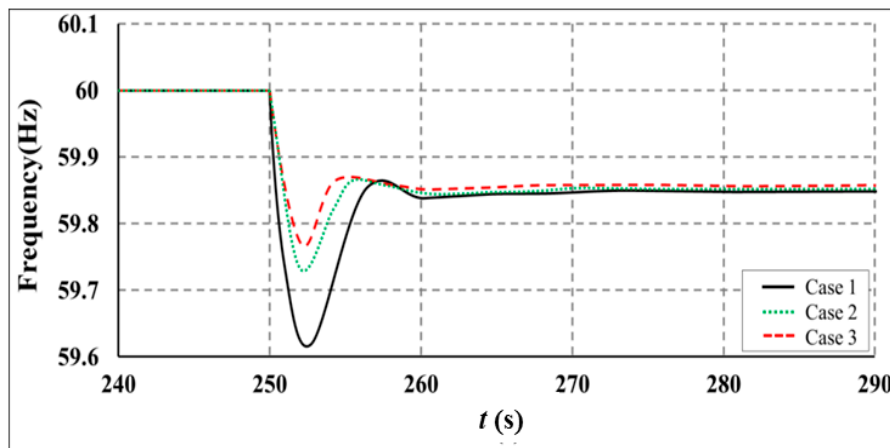
Figure 14. Comparison of the system frequency response.
