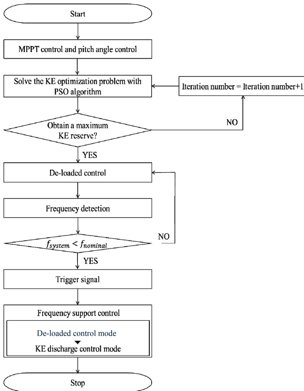
Figure 9. Proposed optimal strategy scheme.
