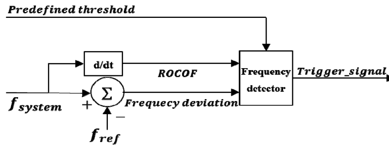
Figure 8. The triggering scheme and frequency detection.
