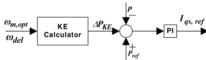
Figure 5. KE reserve controller.
