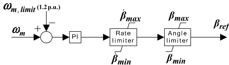
Figure 6. Pitch angle controller.
