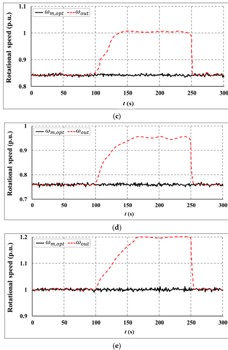
Figure 13. Rotational speed for individual wind farms in Case 3. (a) WF1; (b) WF2; (c) WF3; (d) WF4; (e) WF5.
