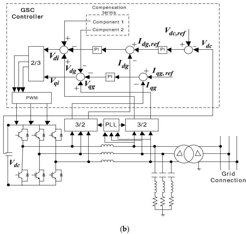
Figure 1. Block diagram of machine-side converter (MSC) and grid-side converter (GSC). (a) MSC control system; (b) GSC control system.
