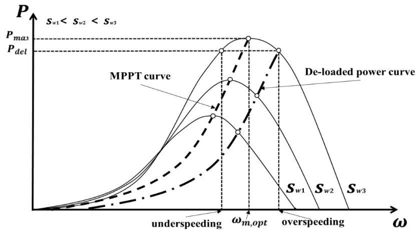
Figure 2. Maximum power point tracking (MPPT) and de-loaded power extraction curves for different wind speeds.
