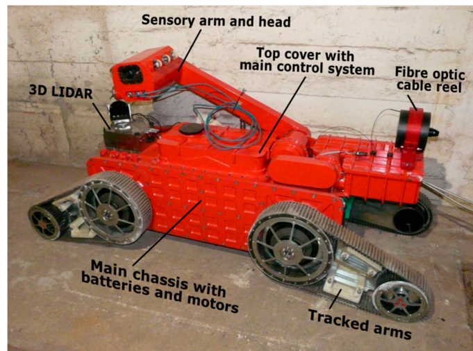
Figure 4. TeleRescuer—main subsystems.
