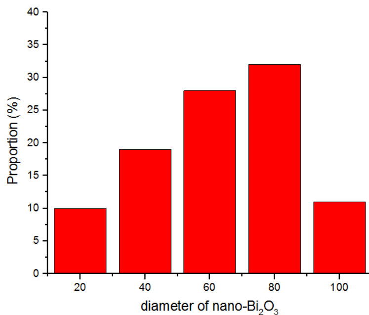
Figure S1. The particle size distribution of nano-Bi 2 O 3
