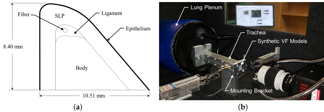
Figure 1. (a) Model of the geometry of the silicone vocal folds; and (b) image of the experimental flow facility.
