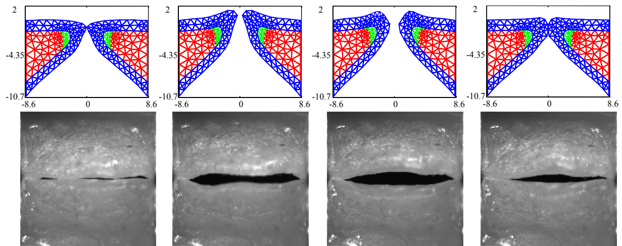
Figure 3. Kinematics of the FE model in comparison with the observed high speed videoendoscopy (HSV) for the case with no medial compression ( p_{sub} = 1 kPa) at several time points throughout a single oscillation cycle.
