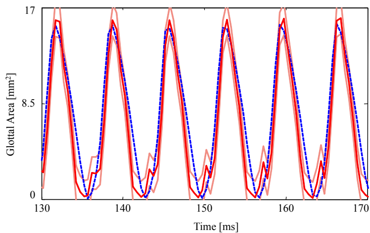
Figure 4. Comparison of the glottal area waveforms extracted from the FE model and the HSV for the case with no medial compression ( p_{sub} = 1 kPa). Blue dashed line: HSV; red solid line: FE model; orange solid lines: uncertainty bounds from the FE estimate.
