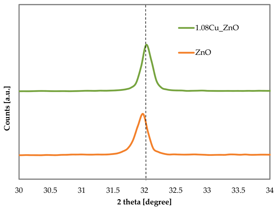
Figure S1. XRD patterns for undoped ZnO and 1.08Cu_ZnO photocatalyst.
