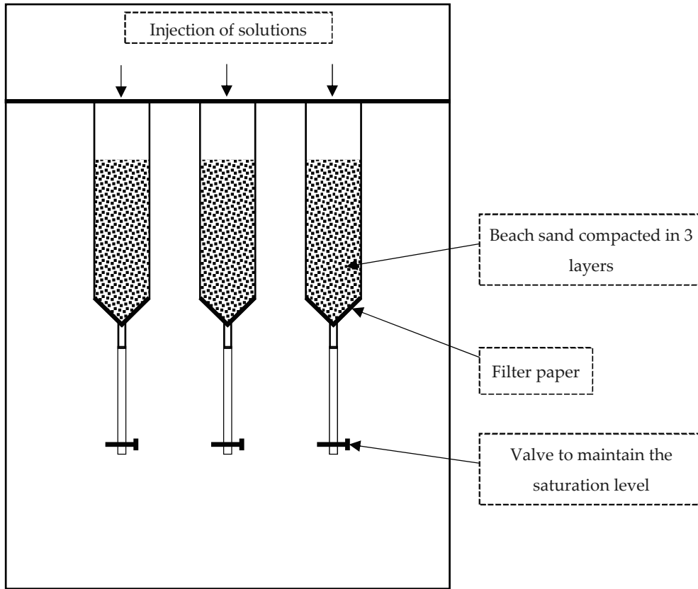
Figure S3: Experimental set up for the syringe sand solidification test.
