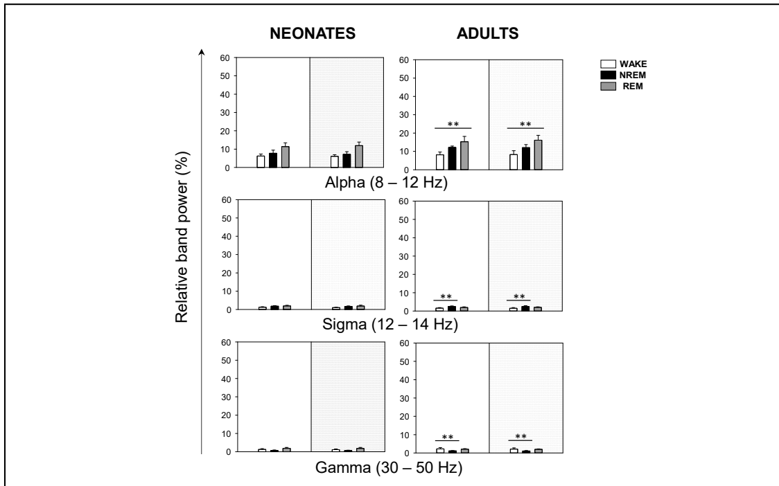
Figure S1. Relative band power of EEG during behavioral states in neonatal and adult mice. Relative band power of EEG in alpha ( \alpha ), sigma ( \sigma ), and gamma ( \gamma ) during behavioral states. Data shown as mean \pm SEM of either 18 or 27 recordings retrieved from 6 neonatal or 11 adult mice, respectively. Asterisks denote significant differences between neonatal and adult mice: ** p < 0.01 ; Two-way ANOVA and Tukey's test for post-hoc analysis.
