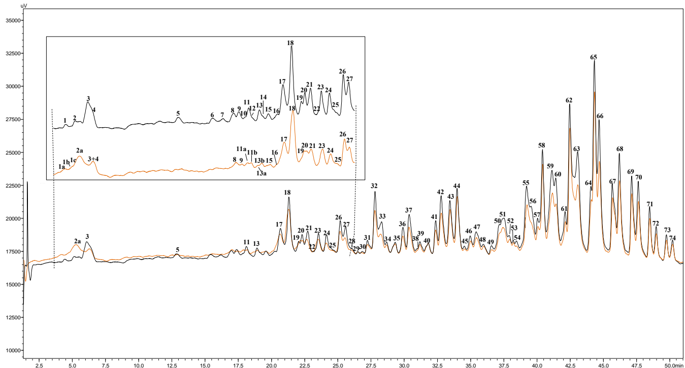
Figure S1. Separation of carotenoids from orange juice before in vitro digestion ( black ) and after in vitro digestion ( orange ) by HPLC-DAD (450 nm). Due to slightly different weights and injection volumes, peak areas are not comparable. Peak assignment is given in Table 3.
