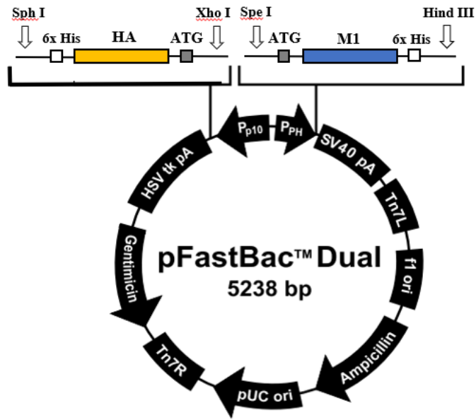
Figure S1. Construction of recombinant plasmid containing the full HA and M1 protein genes. HA and M1 genes derived from the H6 AIV from A/chicken/Taiwan/3943/2012 were cloned into the pFastBac Dual vector.
