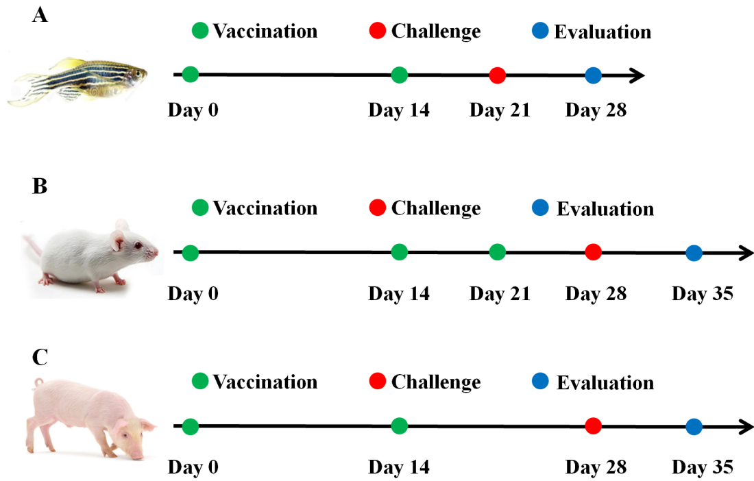
Figure S2 Scheme of the vaccination protocols for (A) zebrafish, (B) mice, and (c) piglets
