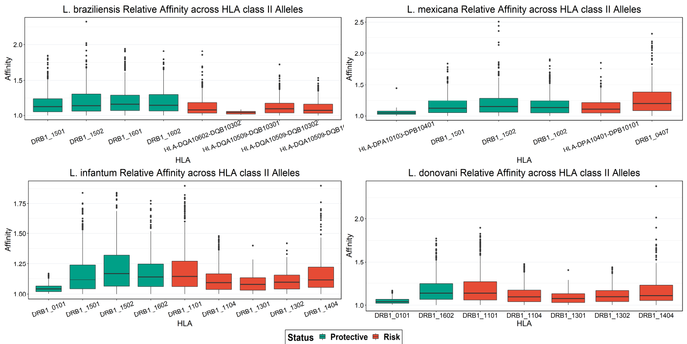
Figure S3. Relative affinity distribution across HLA class II alleles associated with protection and risk for L. braziliensis , L. donovani , L. infantum and L. mexicana .
