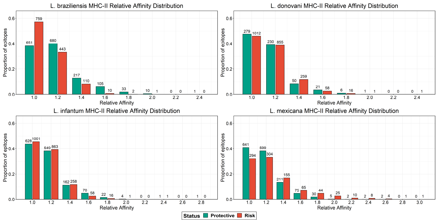
Figure S2. Relative affinity distribution plots for the HLA class II alleles associated with L. braziliensis , L. donovani , L. infantum and L. mexicana . This plot shows the number of epitopes, and the proportion of epitopes relative to the total number of epitopes, with a specific relative affinity.
