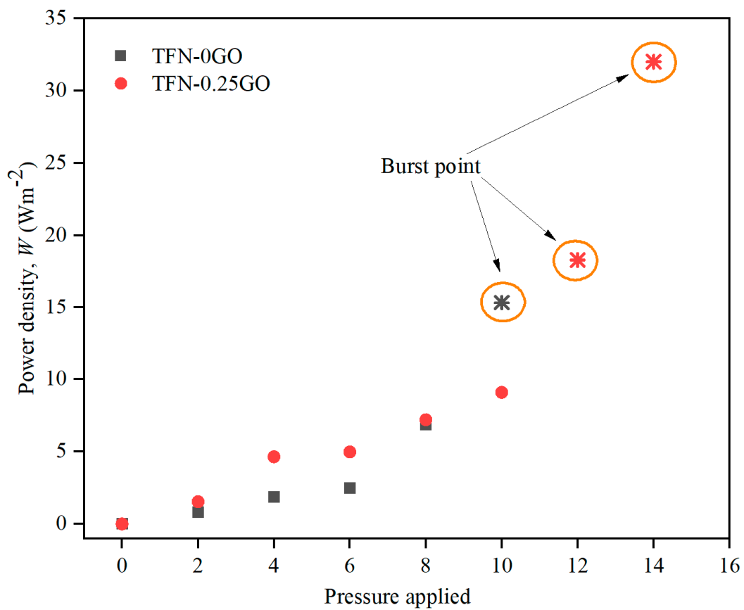
Figure S2. Burst point (membrane damaged) power density of TFN-0GO and TFN-0.25GO.
