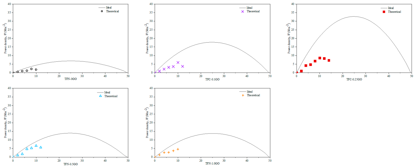
Figure S3. The power density graph of all the TFN-GO membranes.
