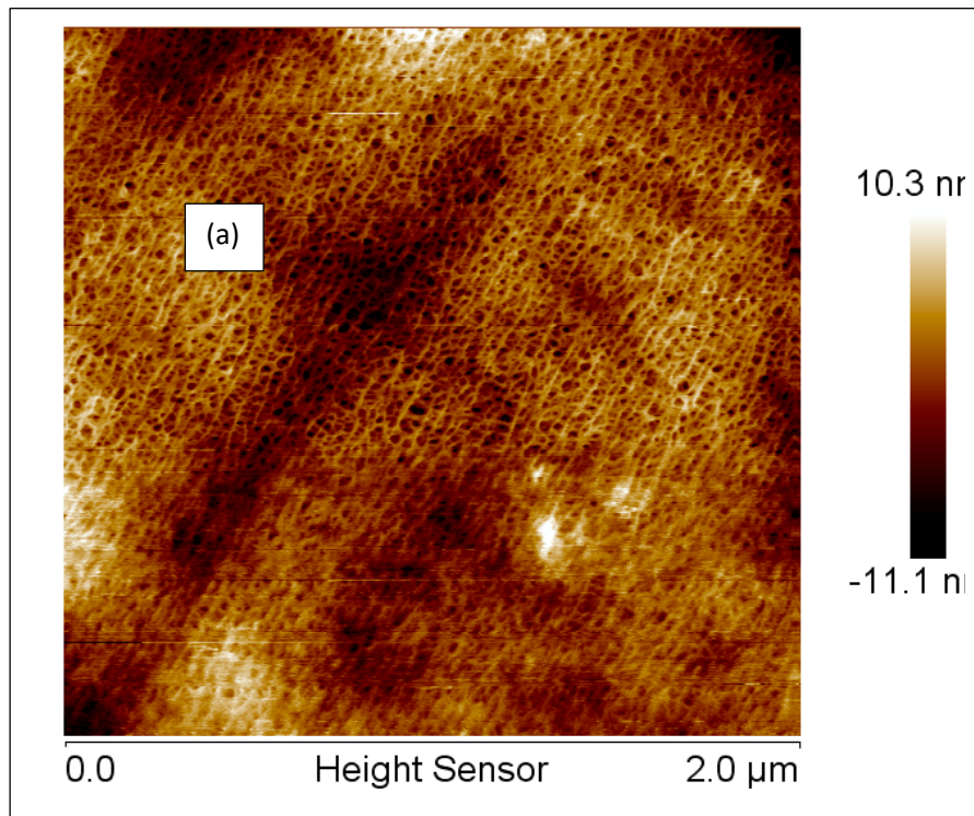
Supplementary Fig. 3: AFM images for 100 kD base RCUF membrane.
