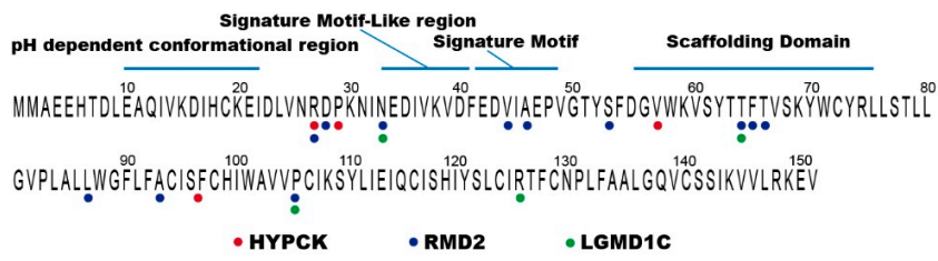
Figure S1: Disease-related amino acids of Cav3. HYPCK, HyperCKemia; RMD2, rippling muscle disease-2; LGMD1C, limb-girdle muscular dystrophy (LGMD) type 1C.
