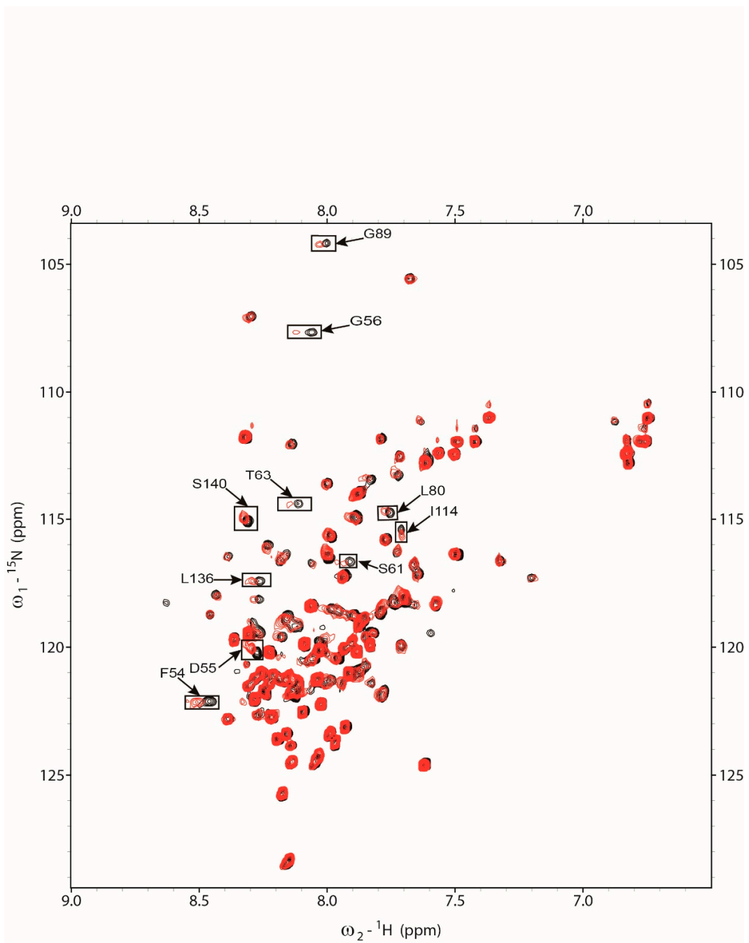
Figure S2: HSQC spectra of Cav3 in LPPG micelle with (red)/without (black) cholesterol.
