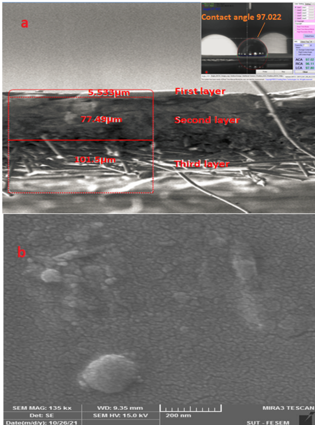
Figure 2. (a) Contact angle of PDMS membrane and SEM image of PDMS membrane cross section (200 μm). (b) SEM image of PDMS membrane surface.
