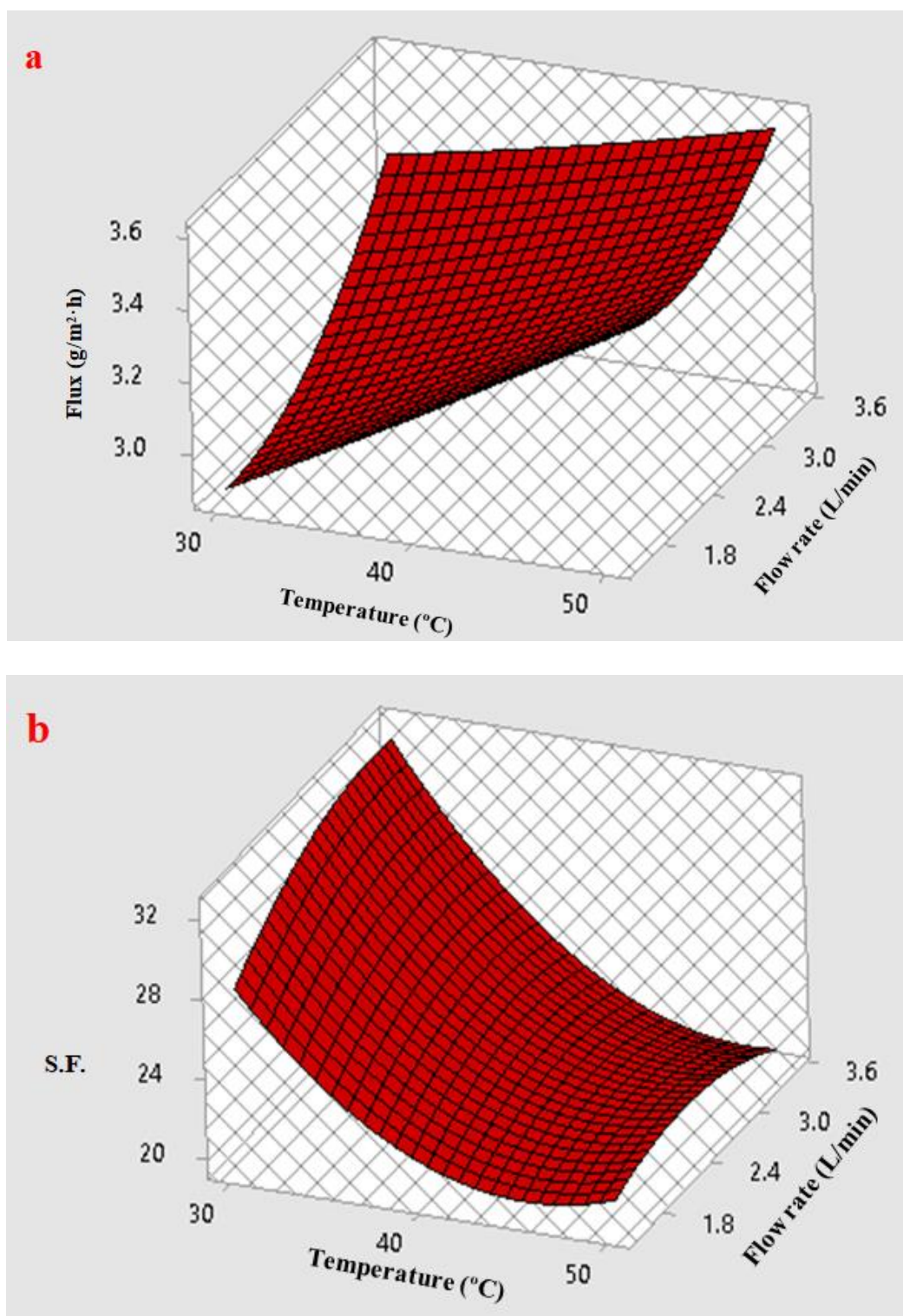
Figure 10. Effect of the feed temperature and feed flow on (a) benzene flux and (b) Separation factor (S.F.) at an initial benzene concentration of 550 ppm.
