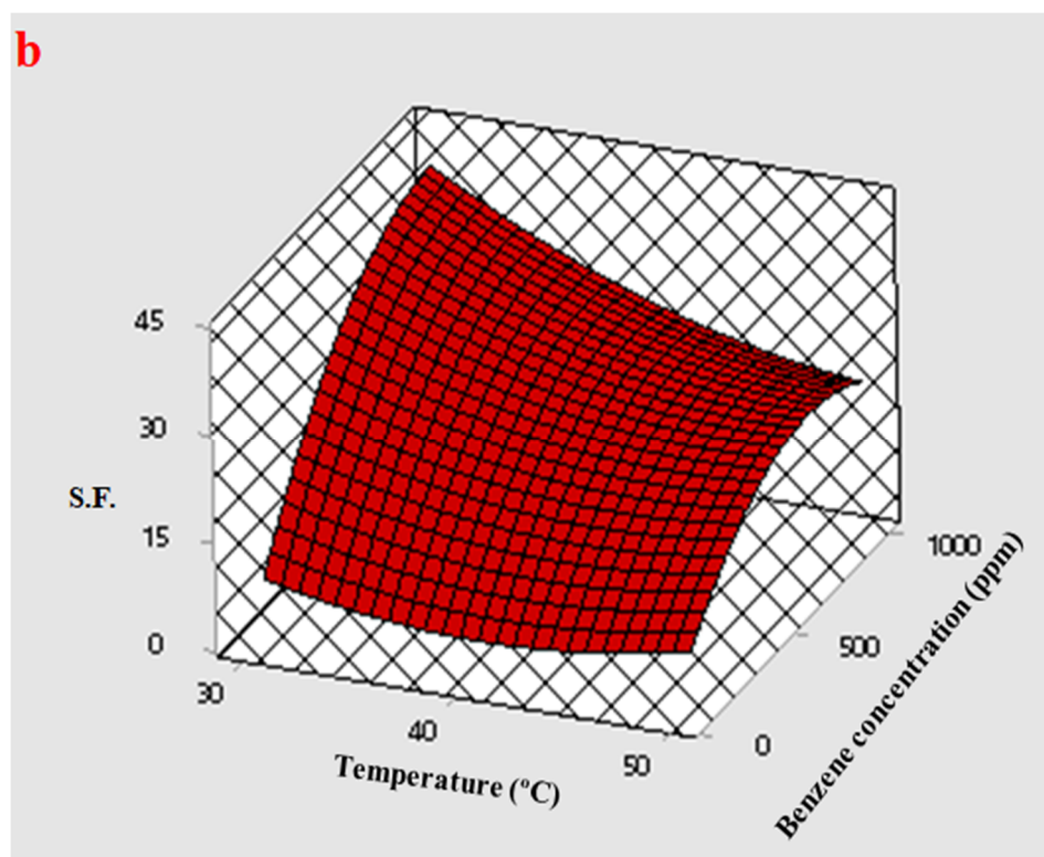
Figure 9. Effect of the feed temperature and the benzene concentration on (a) benzene flux and (b) separation factor (S.F.) at a feed flow rate 2.5 L/min.
