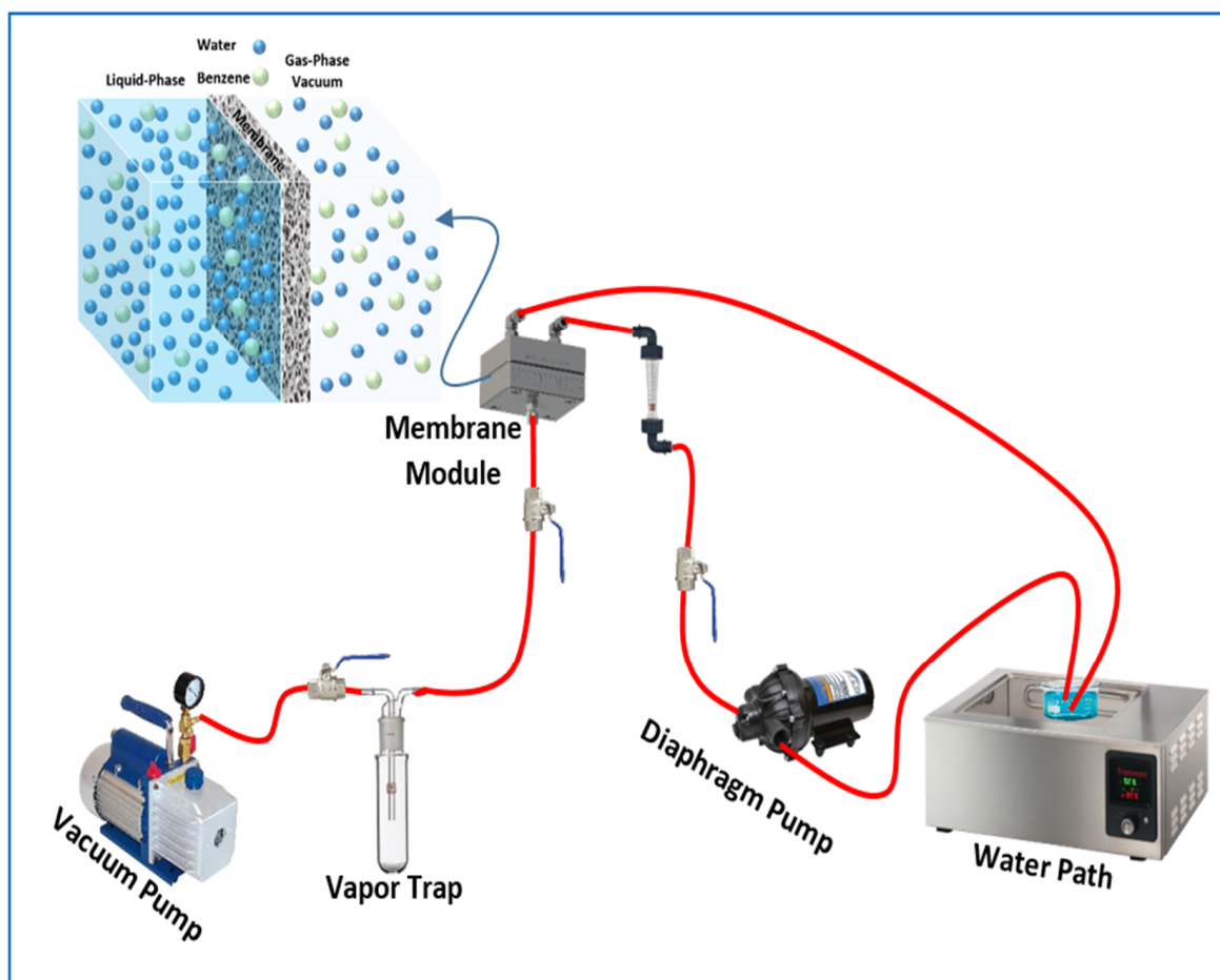
Figure 1. Schematic diagram of the pervaporation process.
