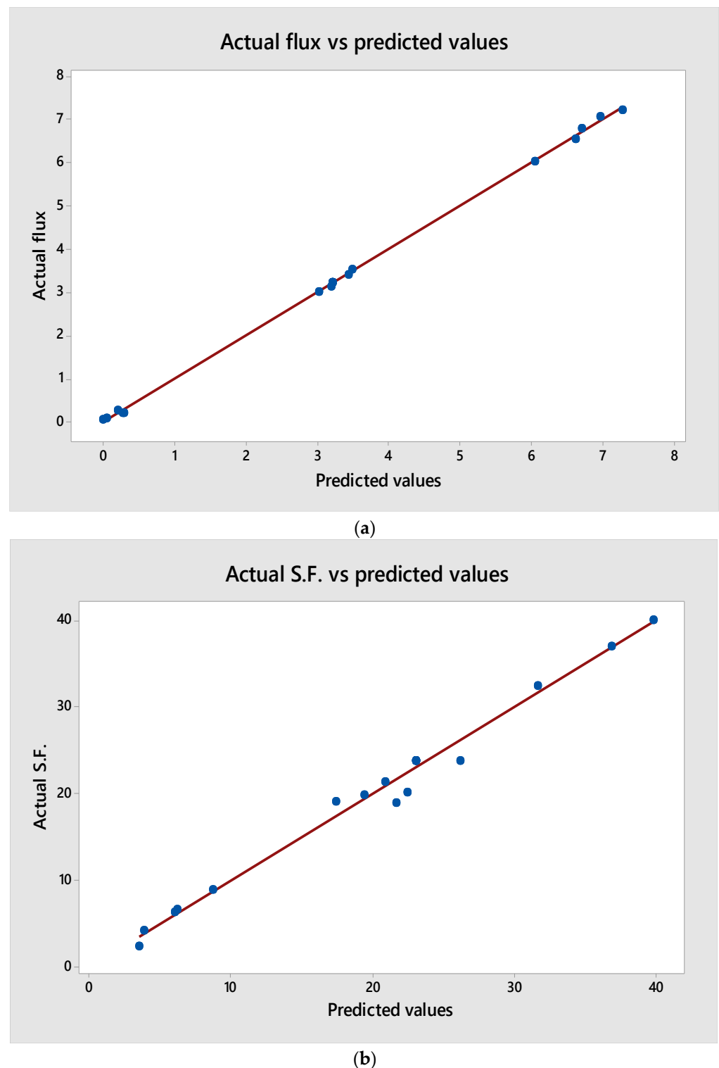
Figure 7. The relationship between the actual and predicted (a) benzene flux and (b) S.F.
