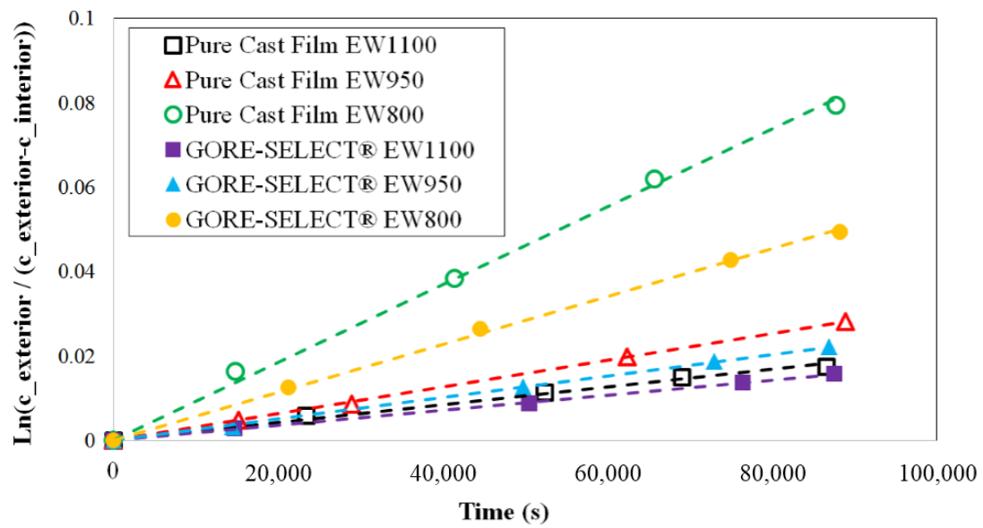
Figure S3. Semi-natural log plot used to determine permeability based on V(IV) ion diffused concentration.
