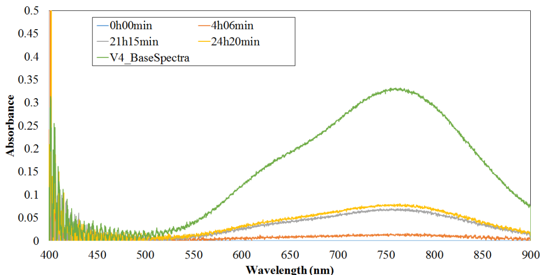
Figure S1. Calibration spectra for detection of the V(IV) ion via UV-Vis spectroscopy.
