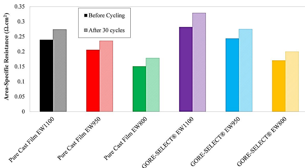
Figure S2. Area-specific resistance ( \Omega \cdot \text{cm}^2 ).
