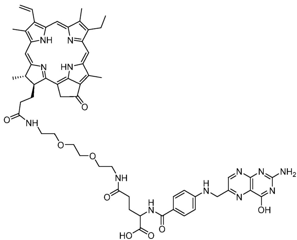
Figure S1. Structural formula of the compound Pyro-PEG-FA (PS2).
