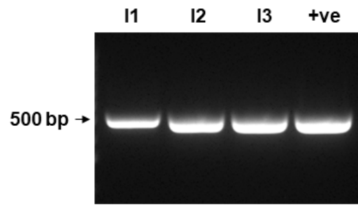
Figure S1. PCR amplification using Ptr specific primers PtrUnique_F2/R2 confirming the fungal colonies with atypical morphology as Ptr. I1, I2 and I3 represent PCR products of three different colonies with similar atypical morphology. DNA of the isolate M4 was used as a positive control for the PCR amplification (+ve).
