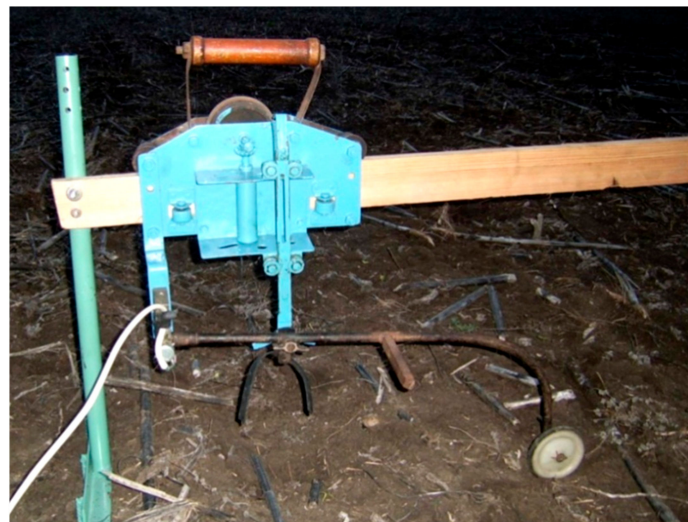
Figure 3. Device for measuring surface profile oscillations.
