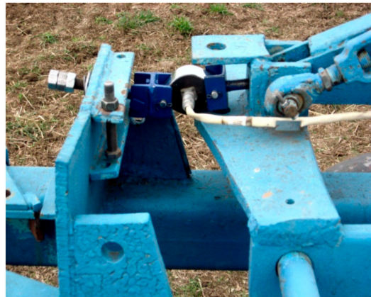
Figure 5. Strain-measuring plough.
