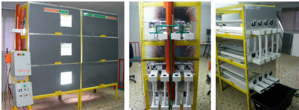
Figure A1. Construction of the Photon Rack (PR) system at K.Dekoulis Lab in Kallithea, Athens, Greece.
