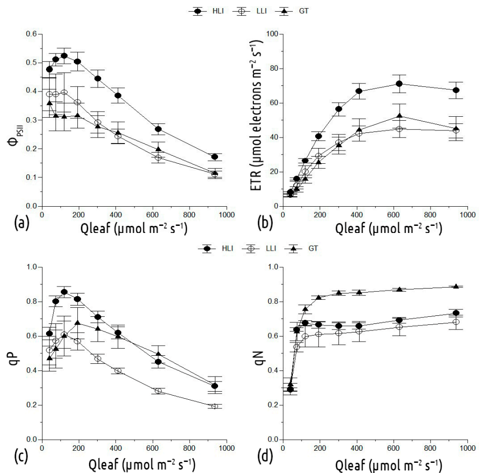
Figure 4. \Phi_{PSII} (a), ETR (b), qP (c) and qN (d) of an average lettuce plant grown under each different treatment. HLI, High light intensity; LLI, Low light intensity; GT, Glasshouse treatment. Vertical bars indicate \pm standard errors of means.
