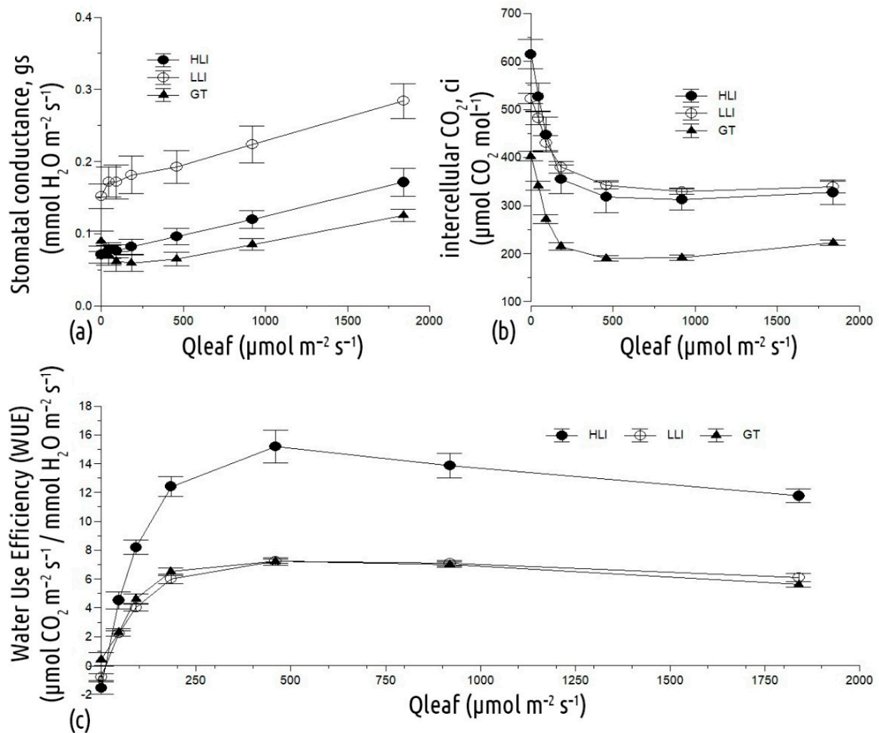
Figure 6. Stomatal conductance, gs, (a) intercellular CO 2 , ci, (b,c) water use efficiency (WUE) of an average lettuce grown under each treatment's conditions. HLI, High light intensity; LLI, Low light intensity; GT, Glasshouse treatment. Vertical bars indicate ± standard errors of means.
