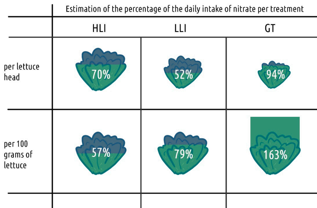
Figure 7. Estimation of percentage of the daily intake of nitrate of each treatment per average lettuce head and per 100 g of fresh produce. HLI, High light intensity; LLI, Low light intensity; GT, Glasshouse treatment.
