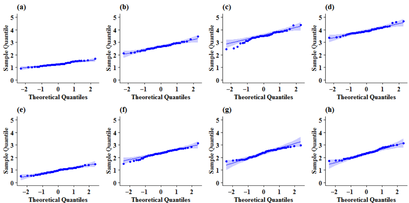
Figure 4. Q-Q results of experimental data. (a) Jointing, 2020; (b) 9th leaf, 2020; (c) Big trumpet, 2020; (d) Silking, 2020; (e) Jointing, 2021; (f) Big trumpet, 2021; (g) Silking, 2021; (h) Blister, 2021.
