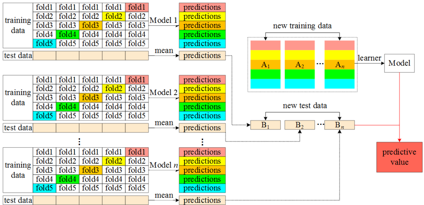
Figure 3. Schematic diagram of stacking algorithm workflow.
