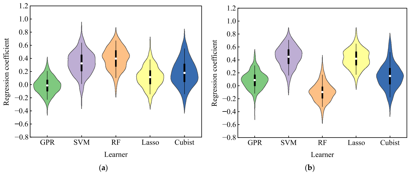
Figure 7. Base model coefficient distribution in secondary models (MLR) in (a) 2020 and (b) 2021.
