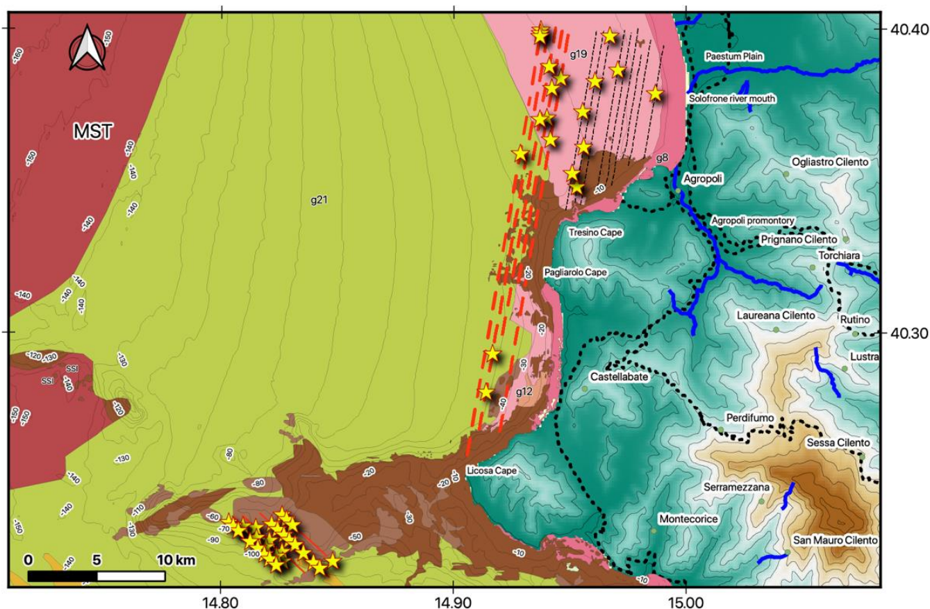
Figure 14. Sketch map showing the distribution of the acoustic anomalies (yellow stars) in the study area based on seismic interpretation.
