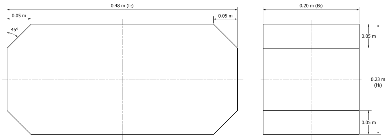
Figure 2. First-angle projection of the open-bore tank geometrical model.
