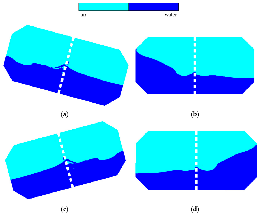
Figure 13. Cross-sectional contoured illustrations of the sloshing dynamics within the perforated-partitioned tank at 40% fill. (a) \theta_t = -15^\circ (initial position). (b) \theta_t = 0^\circ (quarter-stroke). (c) \theta_t = 15^\circ (mid-stroke). (d) \theta_t = 0^\circ (three-quarter-stroke).
