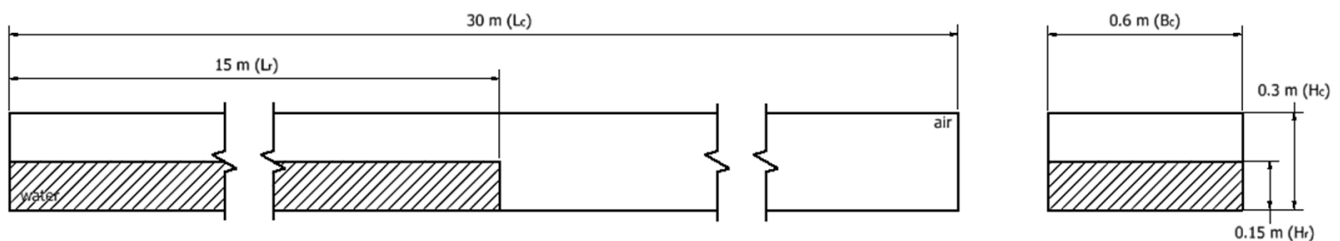
Figure 1. First-angle projection of the dam-break channel geometrical model; shaded volume represents the secondary-phase sub-domain.
