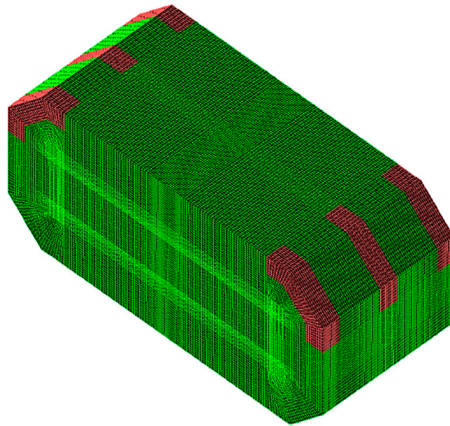
Figure 5. Meshed representation of the open-bore tank with highlighted surface zones for area-averaged static pressure data acquisition.
