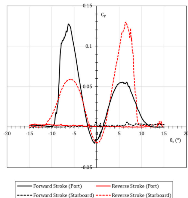
Figure 10. Cycle-averaged pressure coefficient ( C_p ) with angular displacement ( \theta_t ) of the open-bore tank at 40% fill.
