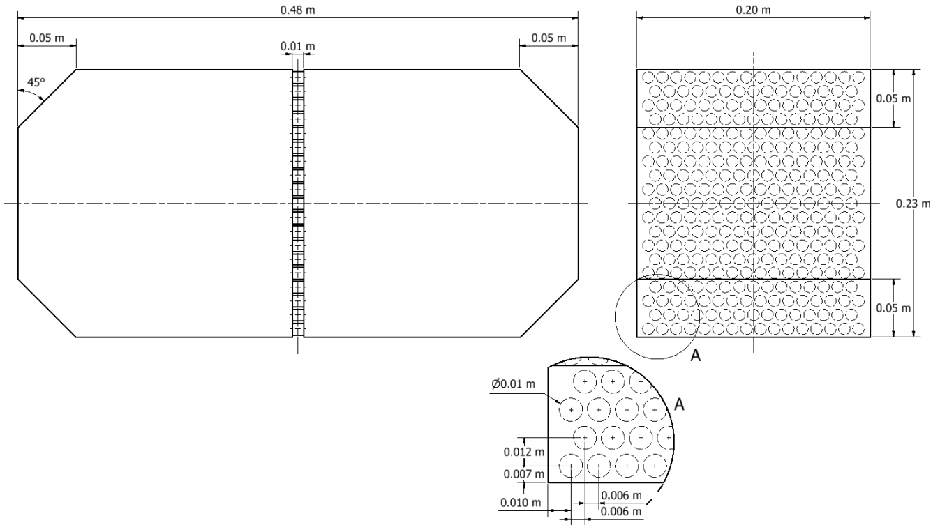
Figure 4. First-angle projection of the perforated-partitioned tank geometrical model.
