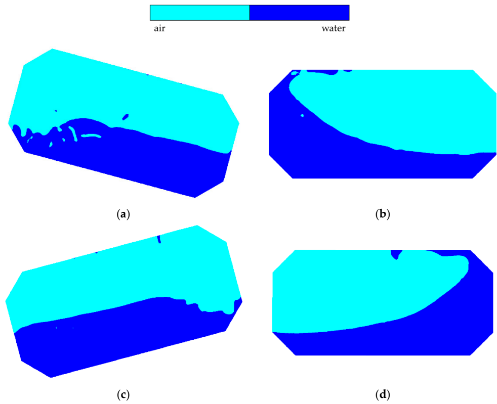
Figure 11. Cross-sectional contoured illustrations of the sloshing dynamics within the open-bore tank at 40% fill. (a) \theta_t = -15^\circ (initial position). (b) \theta_t = 0^\circ (quarter-stroke). (c) \theta_t = 15^\circ (mid-stroke). (d) \theta_t = 0^\circ (three-quarter-stroke).
