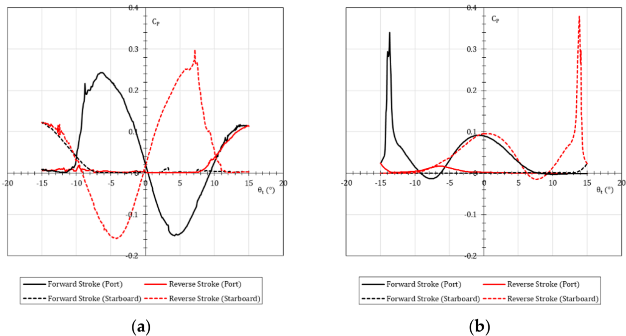
Figure 15. Cycle-averaged pressure coefficient ( C_p ) with angular displacement ( \theta_t ) at 60% fill. (a) Open-bore. (b) Perforated-partitioned.
