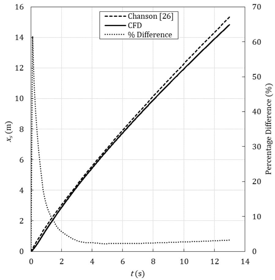
Figure 6. Dam-break wave-tip displacement ( x_s ) comparison between the CFD model and theoretical values derived by Chanson [26].
