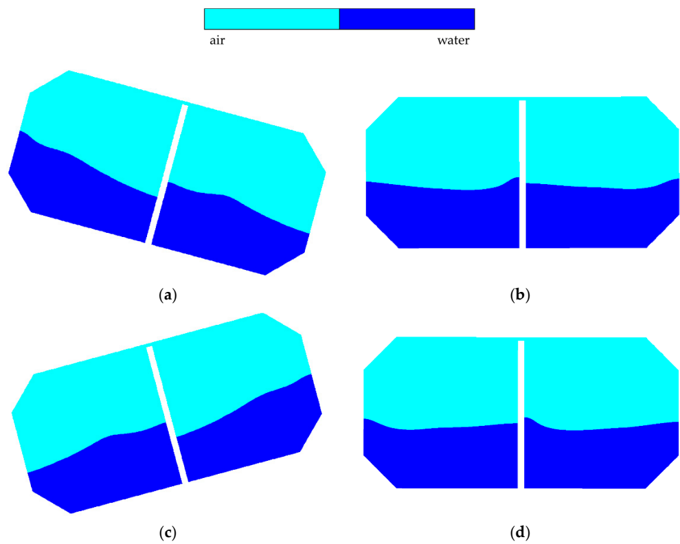
Figure 12. Cross-sectional contoured illustrations of the sloshing dynamics within the partitioned tank at 40% fill. (a) \theta_t = -15^\circ (initial position). (b) \theta_t = 0^\circ (quarter-stroke). (c) \theta_t = 15^\circ (mid-stroke). (d) \theta_t = 0^\circ (three-quarter-stroke).
