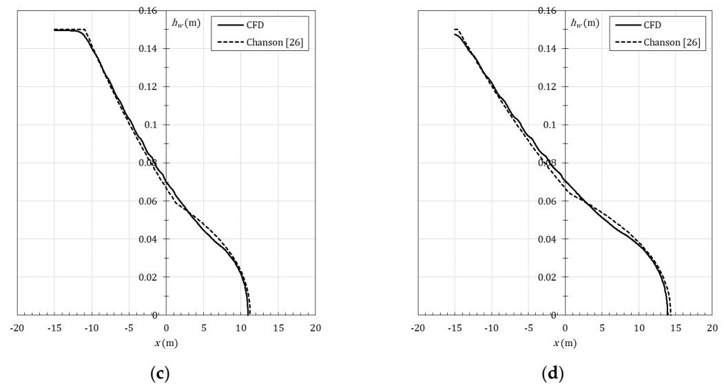
Figure 7. Dam-break free-surface wave profile ( h_w ) comparison between the CFD model and theoretical values derived by Chanson [26]. (a) t = 3 s. (b) t = 6 s. (c) t = 9 s. (d) t = 12 s.
