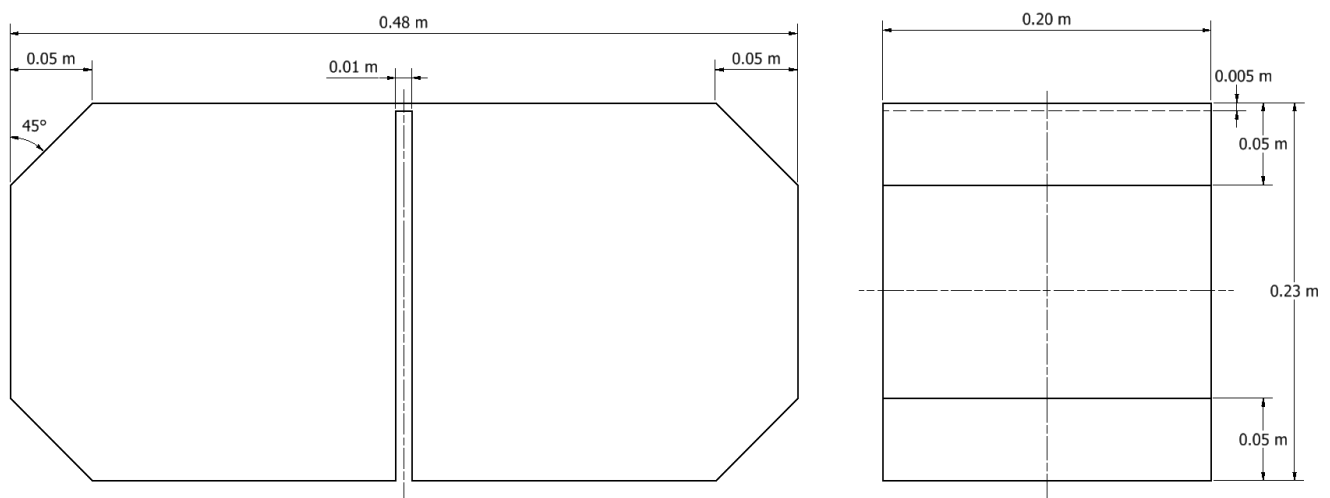
Figure 3. First-angle projection of the partitioned tank geometrical model.
