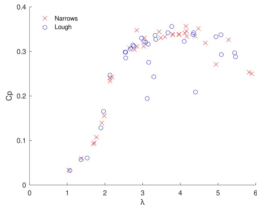
Figure 11. C_p - \lambda data based on filtered steadiest 30 s samples from V1, classified by location, Narrows (energetic) or Lough (still water).
