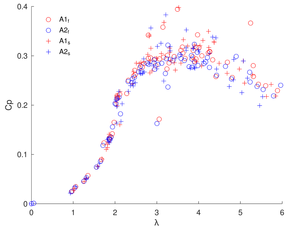
Figure 14. Cp–λ data based on filtered DA and steady A1 data vs A2 data.
