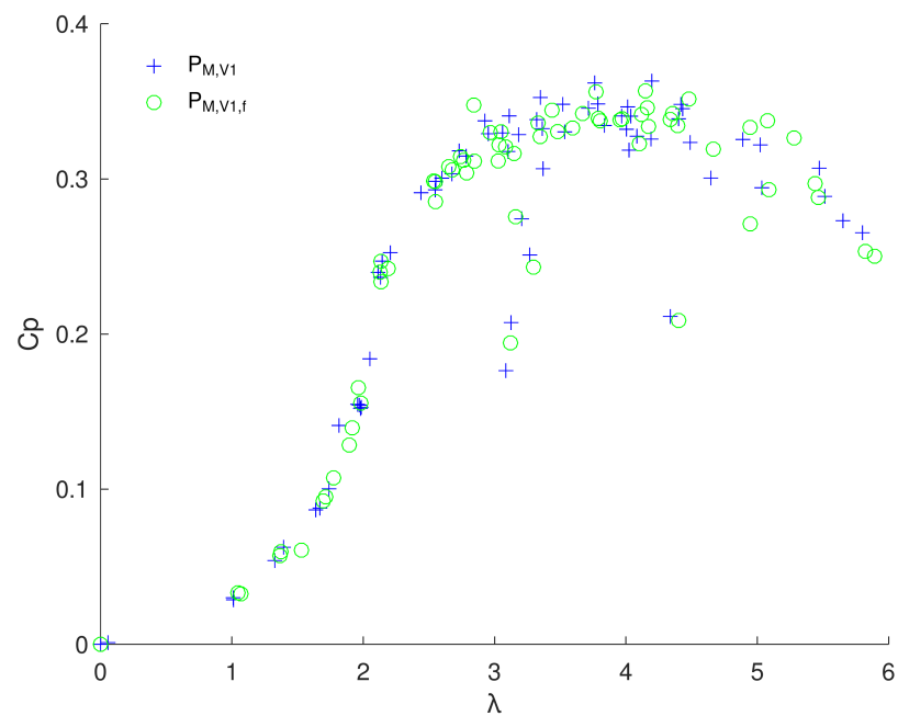
Figure 6. C_p - \lambda data based on mechanical power and Vector1 raw data ( P_{M,V1} ) vs steadiest 30 s sample ( P_{M,V1,f} ).
