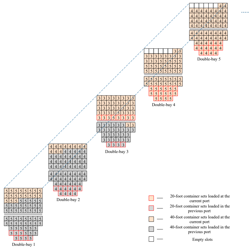
Figure 8. Stowage results in port 2 with rule R2.
