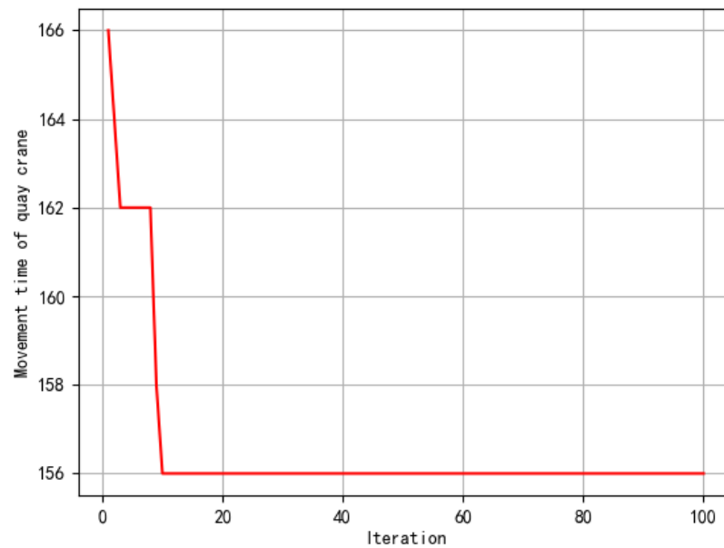
Figure 13. The convergence graph of double-bay.
