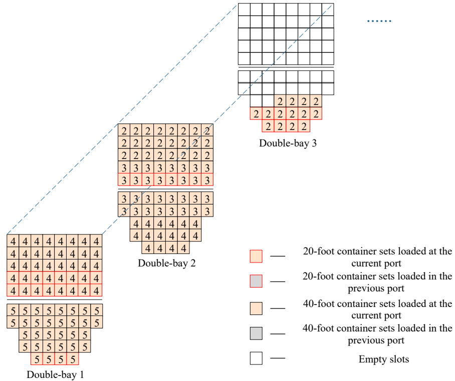
Figure 5. Stowage results in port 1 with rule R1.
