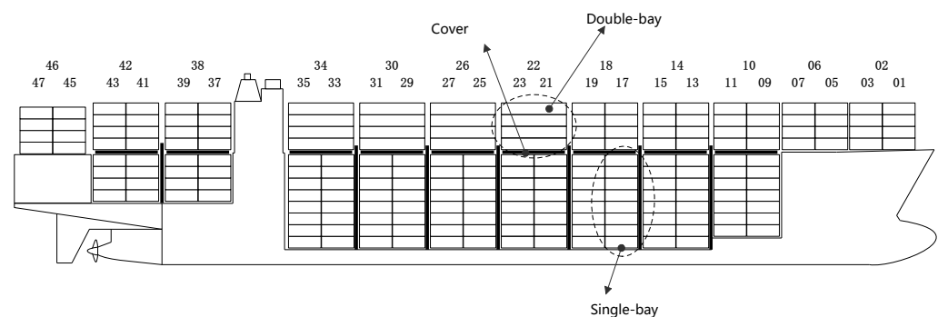
Figure 1. Schematic diagram of the container ship.
