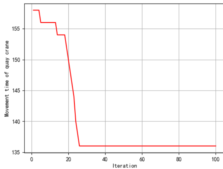
Figure 14. The convergence graph of the single bay.
