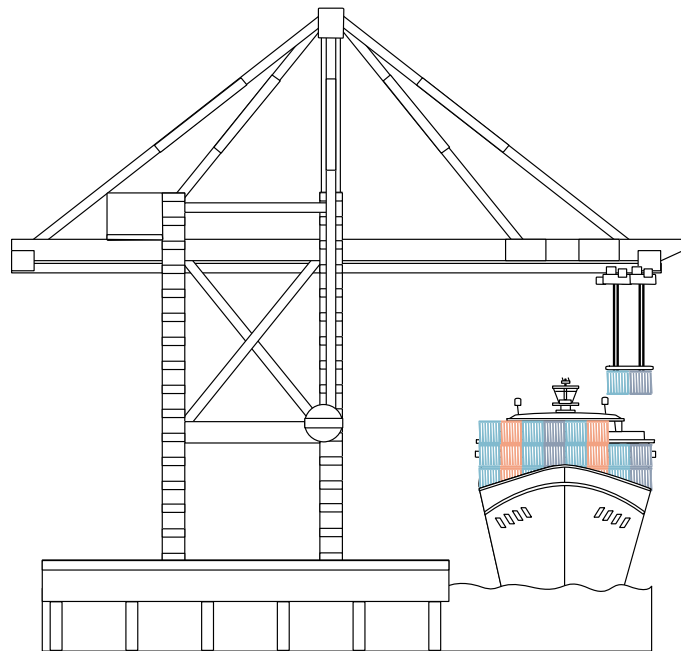
Figure 2. Operation of twin 40-foot QCs with the same tier.
