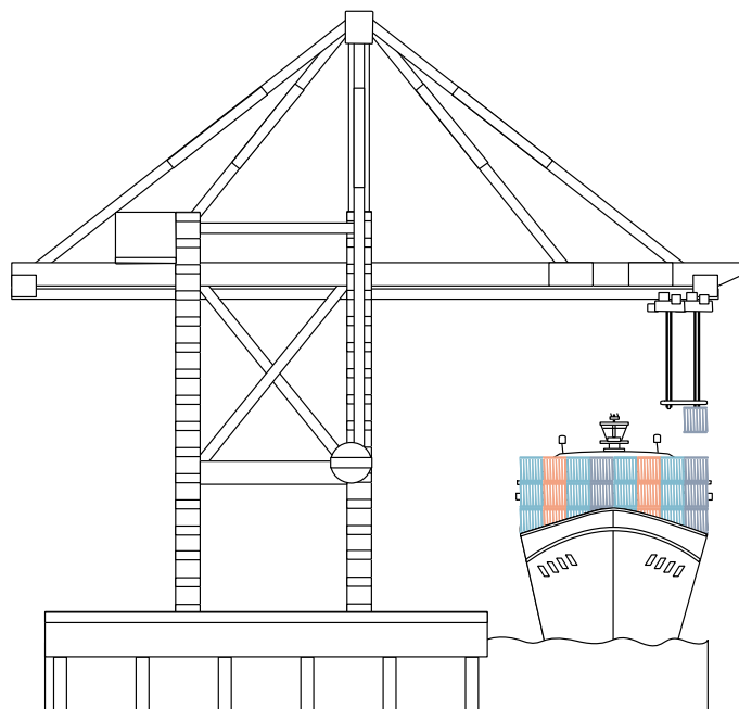
Figure 3. Operation of twin 40-foot QCs with different tiers.
