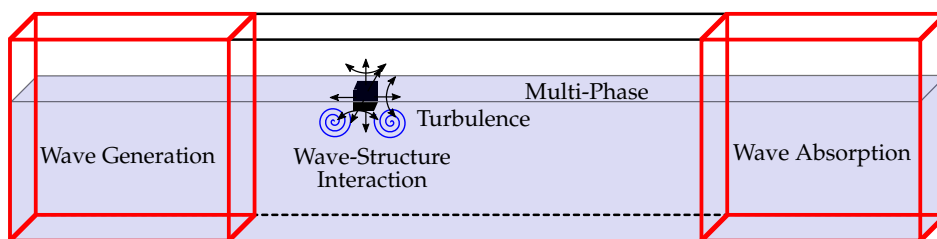
Figure 1. Generic CFD-based numerical wave tank schematic, depicting the main features to be included in the numerical model.
