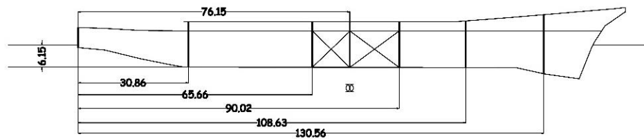
Figure 10. DTMB5415 subdivision and flooded compartment definition—dimensions are in ship scale.
