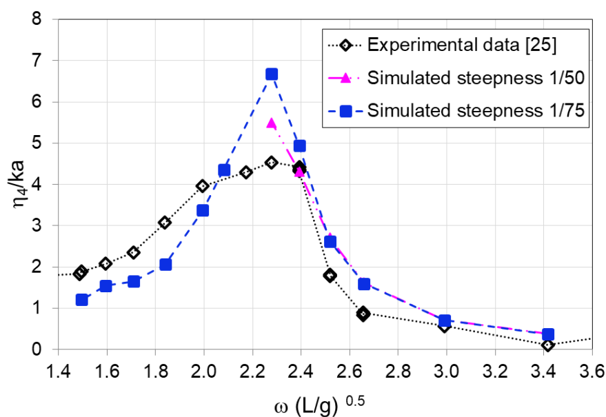
Figure 11. Roll RAO in beam wave: comparison between experimental and simulated results.
