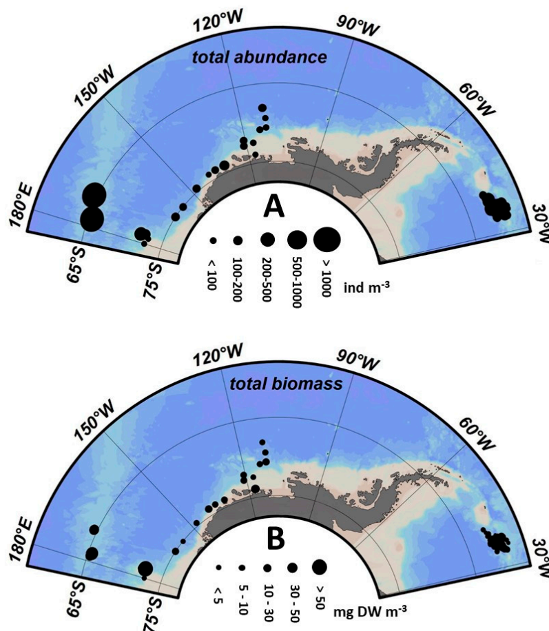
Figure 2. Spatial distribution of total zooplankton abundance ((A), ind m -3 ) and biomass ((B), mg DW m -3 ) in the upper 100 m layer during austral summer 2017–2018 in the Pacific and Atlantic sectors of the Southern Ocean.
