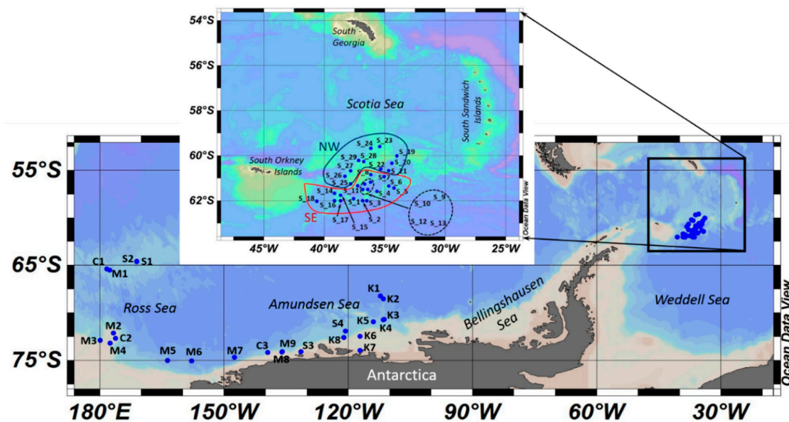
Figure 1. Sample collections carried out from Ukrainian long-liners during austral summer 2017–2018 in the Pacific and Atlantic sectors of the Southern Ocean. In the insert, SIMEIZ collections, NW, northwestern South Orkney Islands (27 February to 3 March, 2018); SE, southeastern South Orkney Islands (31 March to 10 April, 2018). Station abbreviations: K, Koreiz collections (17 November, 2017 to 28 January, 2018); M, Marigolds collections (28 November, 2017 to 24 January, 2018); C, Calypso collections (12 December, 2017 to 18 January, 2018); S, Simeiz collections (29 November, 2017 to 28 January, 2018).
