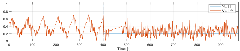
Figure 4. Shows Q_{in} and V_{top} during experiment 1. V_{top} starts fully open and reduces its opening degree to 20% open at 400 s. As a result, the slug is eliminated.
