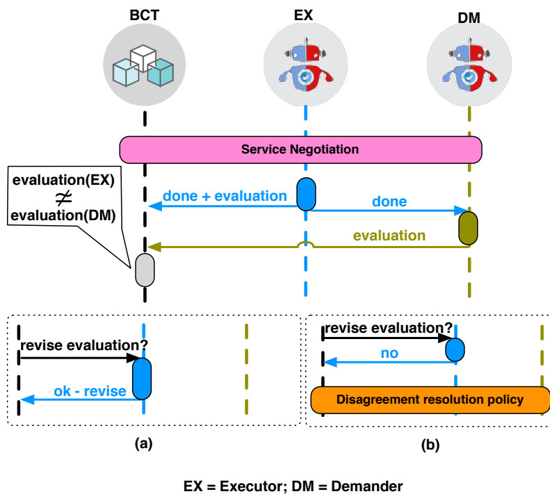
Figure 9. Evaluation management via BCT [9]. (a) computed and the ledger updated, (b) disagreement resolution process is started.
