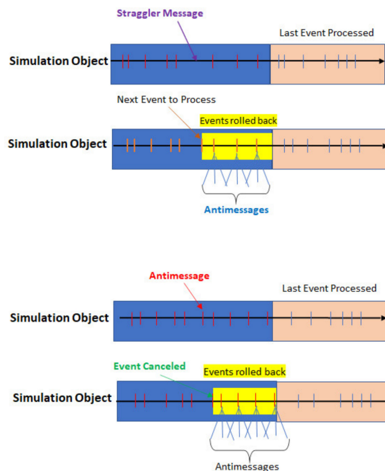
Figure 2. The implementation of rollback produced by straggler messages and antmessages in time warp (TW).
