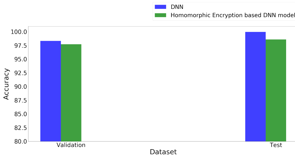
Figure 5. Accuracy-wise performance of the proposed methodology.
