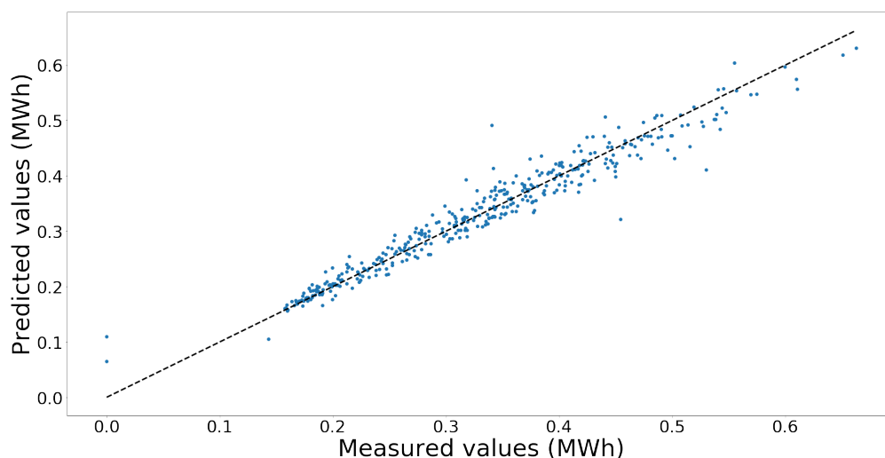
Figure 7. Predicted and actual values of load demand.
