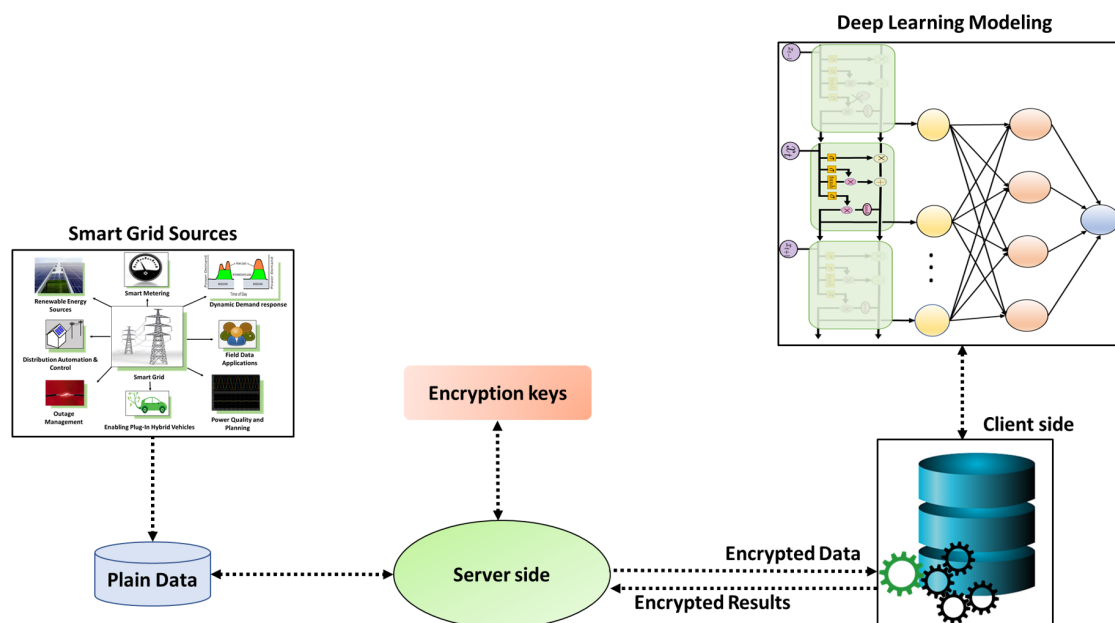
Figure 2. Homomorphic encryption-based deep learning modeling for smart grid applications.
