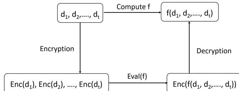
Figure 4. Homomorphic Encryption Evaluation.
