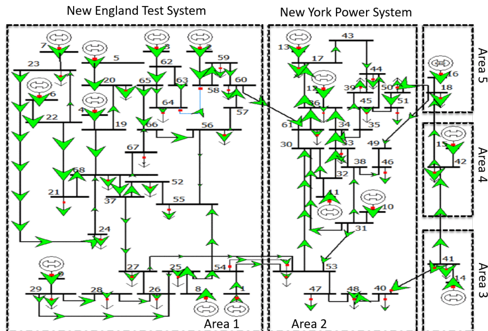
Figure 3. IEEE 68-bus system test simulation model.
