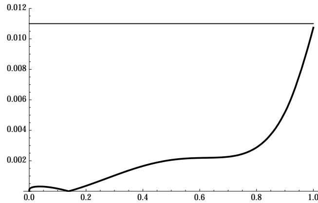
Figure 2. Relative error (in absolute value) \varepsilon_r(y) (9) of a^{-1}_{\text{Vatta-np}}(y) .
