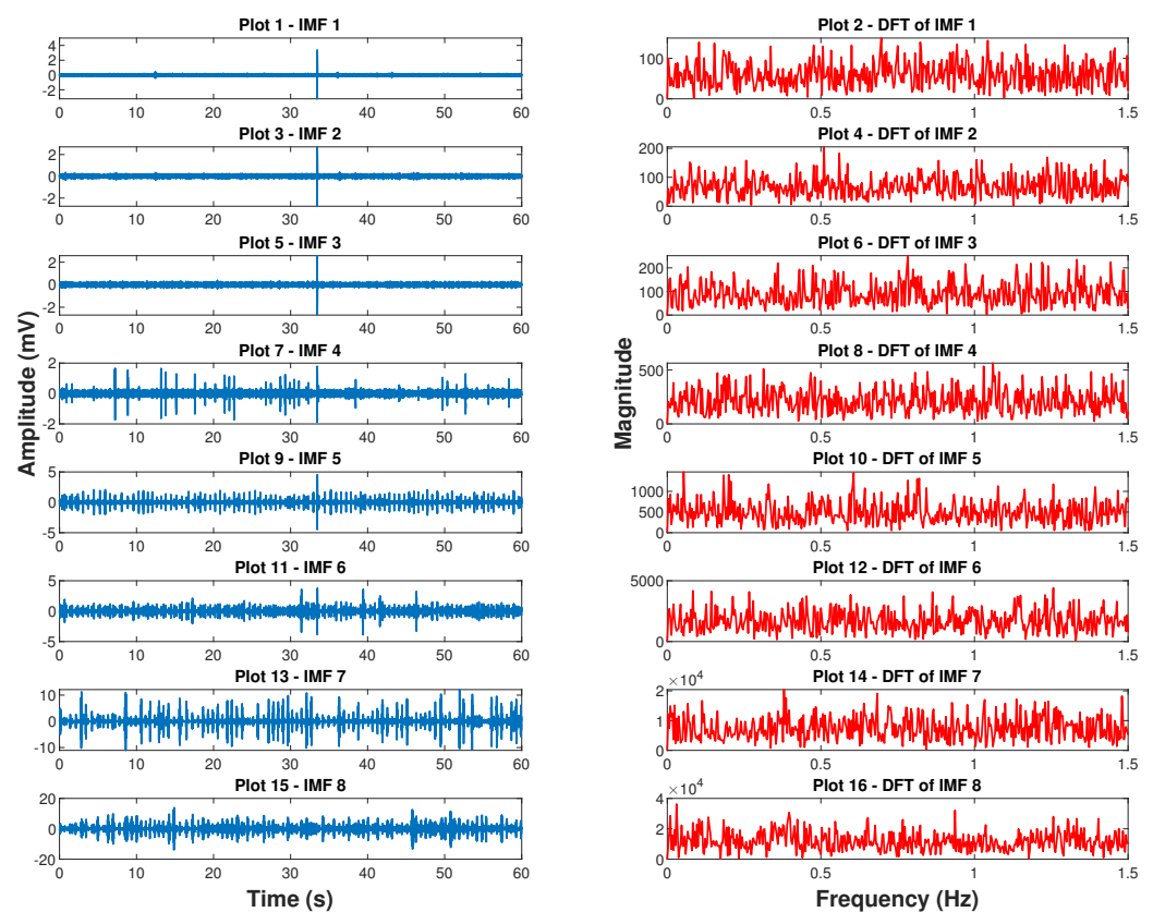
Figure 2. DFT analysis of the IMFs 1 to 8 of b001: The plots on the left column depict IMFs 1 to 8. The plots on the right column show the corresponding spectra (DFT points = 300,000).
