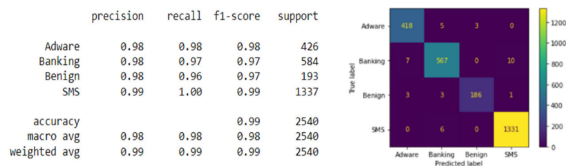
Figure 20. The classification results and confusion matrix for the Random Forest Classifier—API Calls, permissions, and contextual features.
