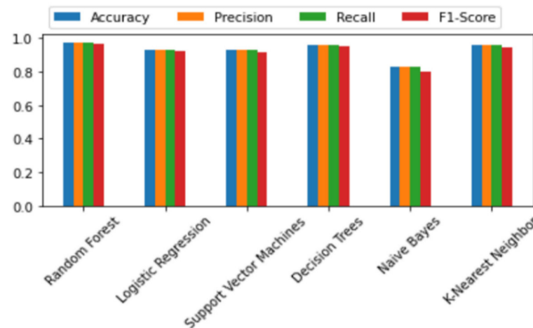
Figure 17. Machine learning classifiers results in detecting Android malware—API Calls with permissions (with feature selection).
