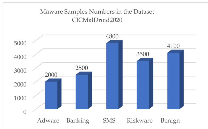
Figure 5. Dataset description.
