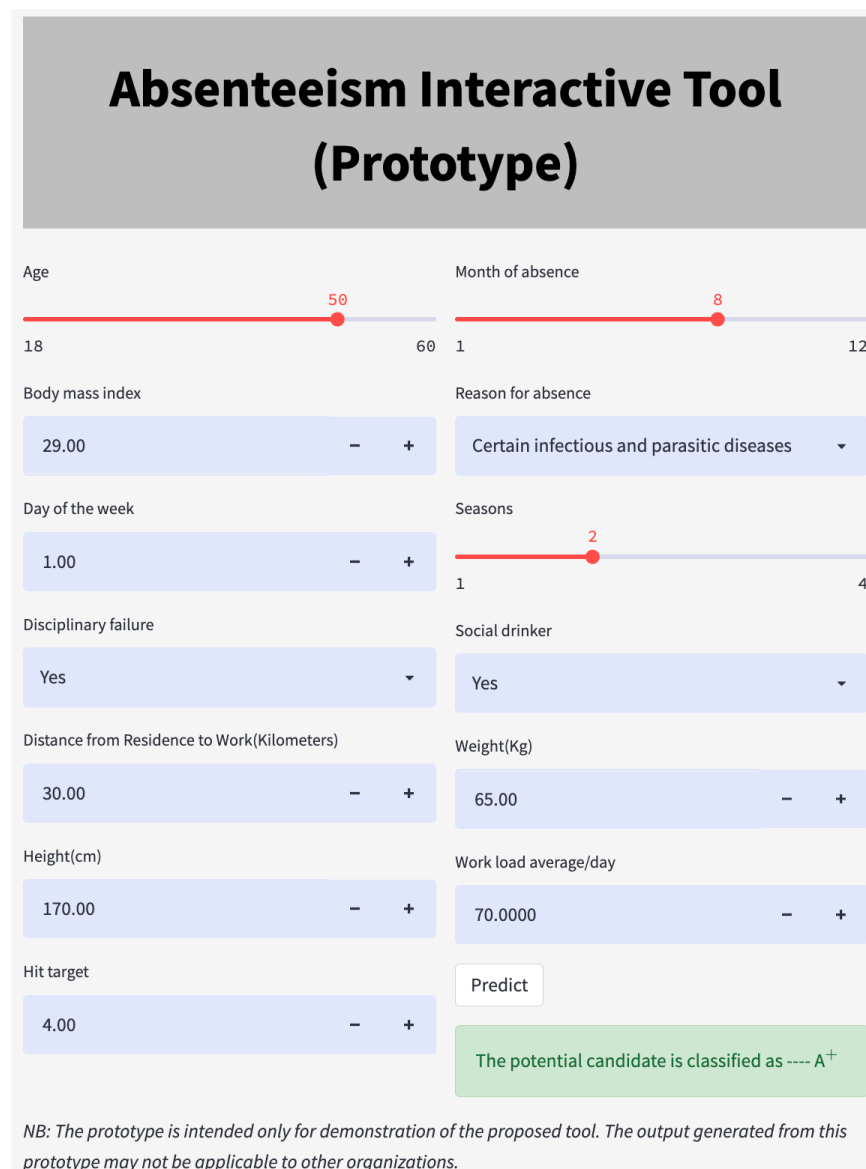
Figure 5. A screenshot of the prototype. Based on input values, the tool classifies the employee as A^+ on a scale of A^+B^+C^+ . The web-based tool is accessible at https://share.streamlit.io/gopalnath1926/app_absenteeism_new/main/app_absenteeism.py (accessed on 24 June 2022).
