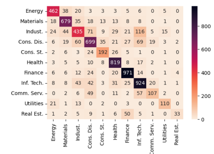
(f) One-vs-Rest with the instructor-large model
