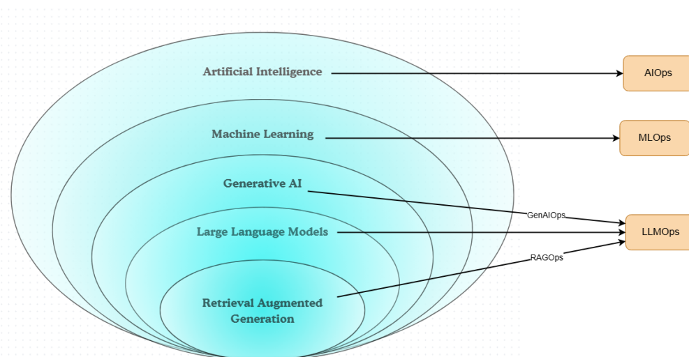
Figure 1. A hierarchy of AI types and associated Ops organized by the level of specialization [57].
