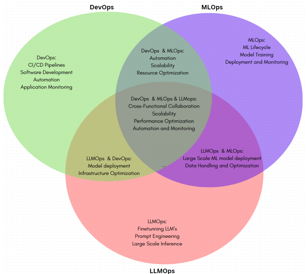
Figure 9. Intersection diagram comparing DevOps, MLOps, and LLMOps [221].
