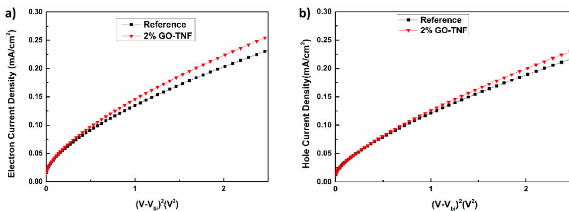
Figure S12. J - V^2 characteristics of the fabricated a) electron-only and b) hole-only devices. The black line refers to the control device (PTB7:PC 71 BM), while the red line corresponds to the ternary PTB7:GO-TNF (2%):PC 71 BM.
