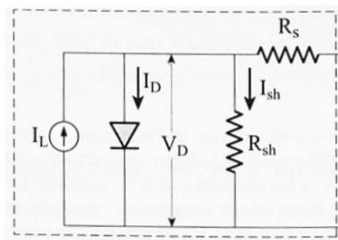
Figure S13. The one diode equivalent circuit model corresponding to the ternary OSC device incorporating 2% GO-TNF ink.
