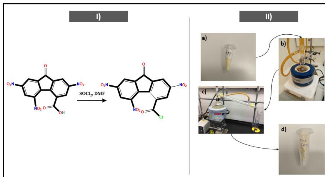
Figure S6. Schematic representation of TNF-COCl synthesis. ii) TNF in powder form (a), the reaction setup b), the distillation setup (c), TNF-COCl in powder form (d).
