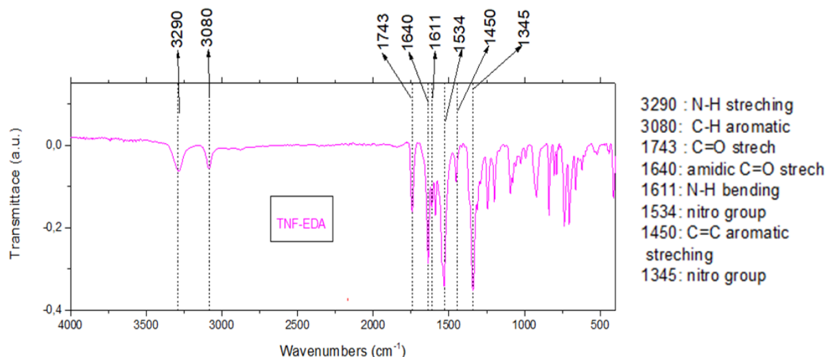
Figure S8. ATR FT-IR spectrum of TNF-EDA.
