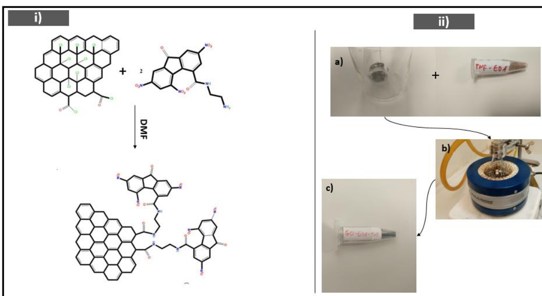
Figure S10. i) Schematic of the final reaction of GO-TNF. ii) GO-COCl and TNF-EDA in powder form (a), setup of the reaction (b), GO-TNF in powder form (c).
