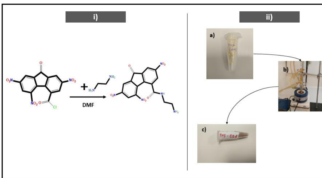
Figure S7. The reaction representation of TNF-EDA synthesis. ii) TNF-COCl powder (a), the reaction setup (b), TNF-EDA in powder form (c).
