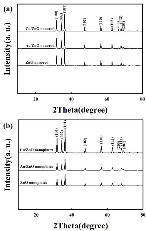
Figure S2. XRD patterns of the samples
