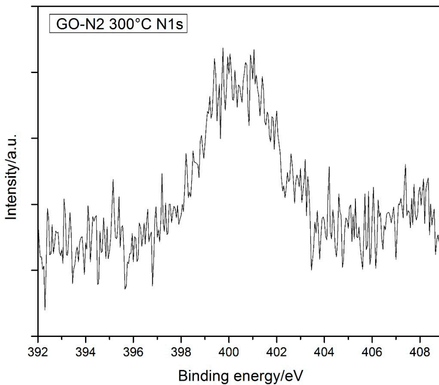
Figure S6 N1s peak for sample GO-N2 300°C
