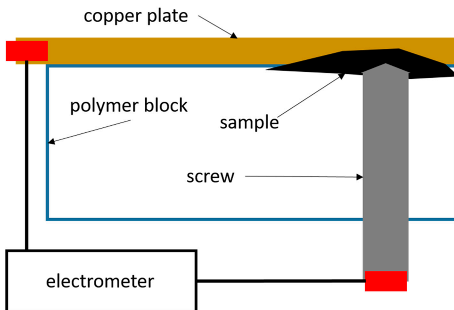
Figure S1 Schematic picture of the electrical resistance measurement setup
