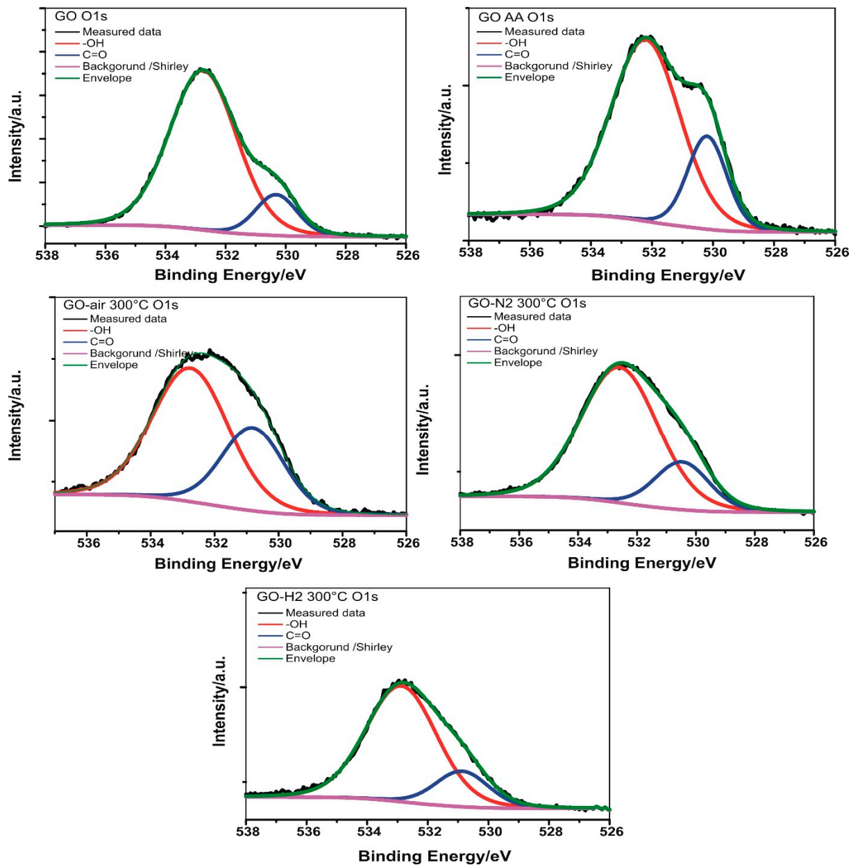
Figure S5 Deconvolution of the O1s peaks for five samples
