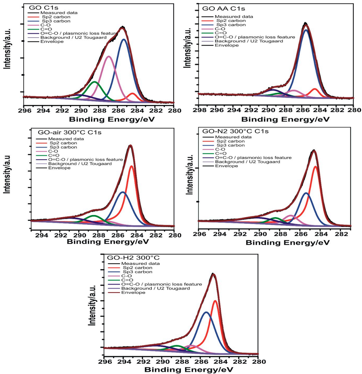
Figure S4 Deconvolution of the C1s peaks for five samples
