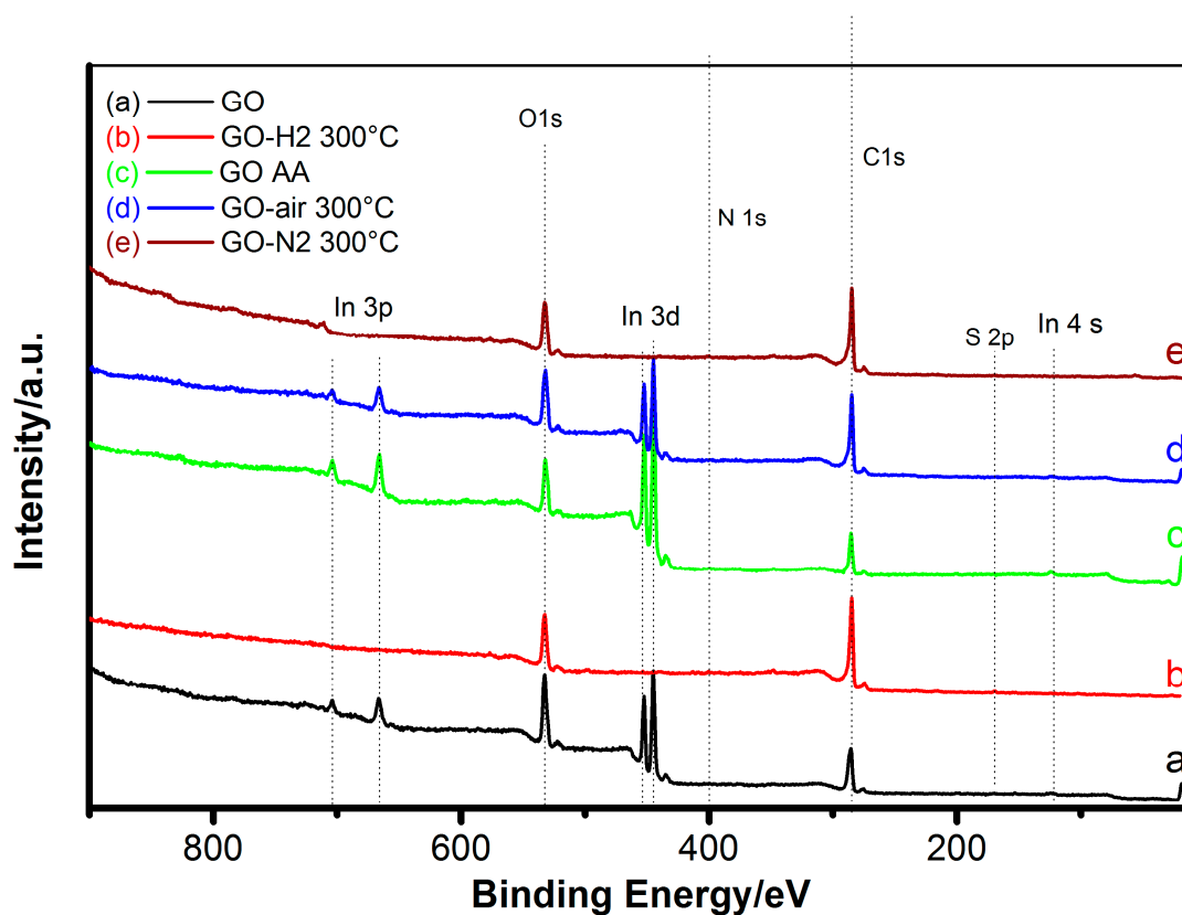
Figure S3 XPS survey spectra for five samples
