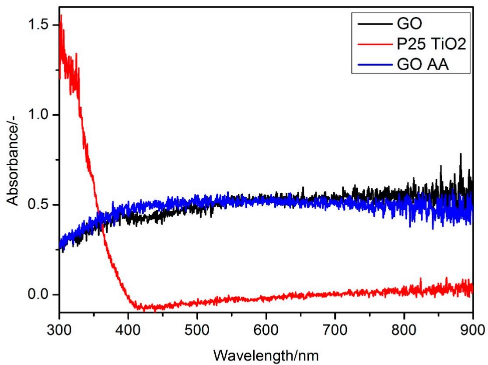
Figure S7 UV-Vis reflectance spectra for GO, GO AA and P25 TiO 2
