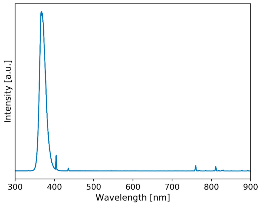
Figure S2 Spectrum of the UV lamp used for the photocatalytic experiments
