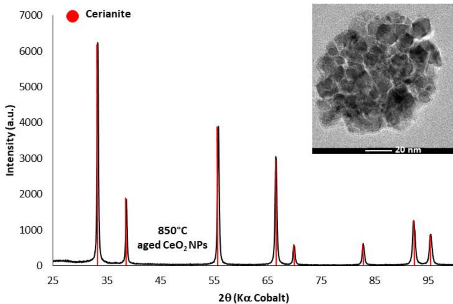
Figure SI1: X-ray diffractogram and transmission electron microscopy image of the 850°C aged CeO 2 NMs.
