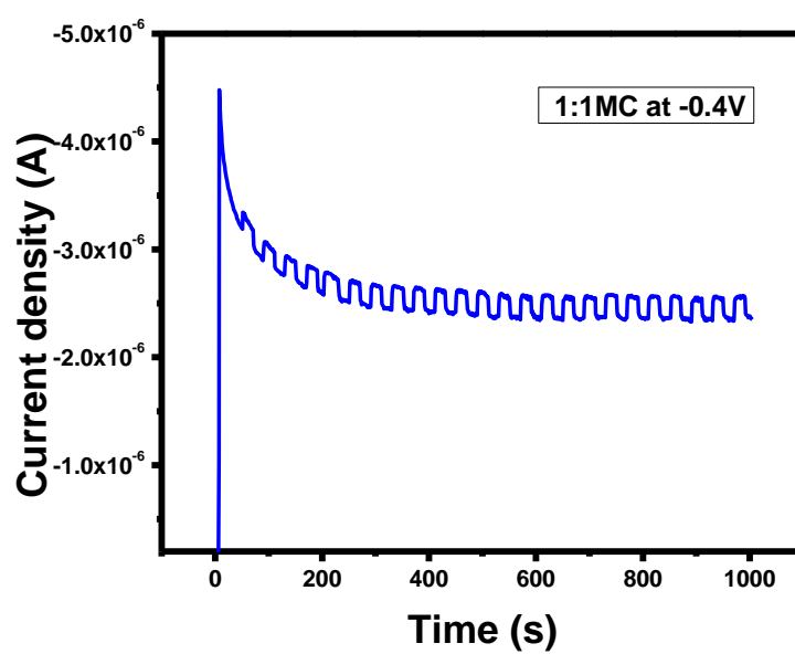
Figure S4. Chronoamperometric response of light on/off for 1:1 MC.
