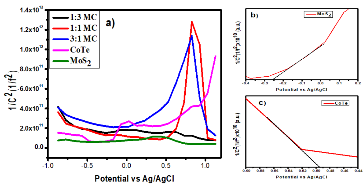
Figure S3. Mott-Schottky plot of (a) MoS 2 , CoTe, 3:1 MC, 1:1 MC and 1:3 MC (b) MoS 2 and (c) CoTe.
