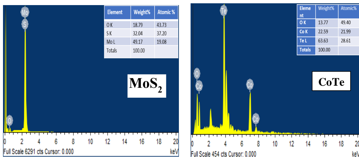
Figure S2. EDS spectra of MoS 2 , CoTe, 3:1 MC and 1:3 MC.
