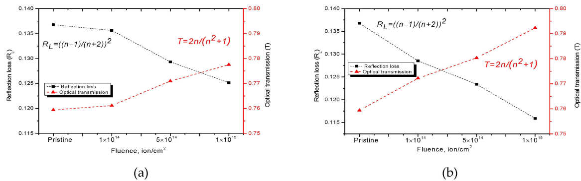
Figure 7. Reflection loss R_L and optical transmission T for: (a) the Kr 15+ ion irradiated dose; (b) the Xe 22+ ion irradiated dose.
