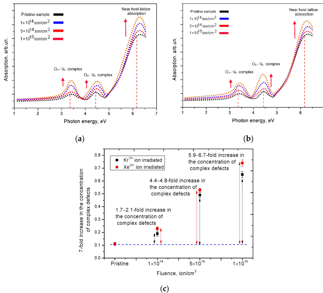
Figure 8. UV-Vis absorption spectra of ceramics before and after irradiation: (a) Kr 15+ ion irradiated dose; (b) Xe 22+ ion irradiated dose; (c) Semi-quantitative analysis of the concentration of complex defects depending on the type of irradiation.
