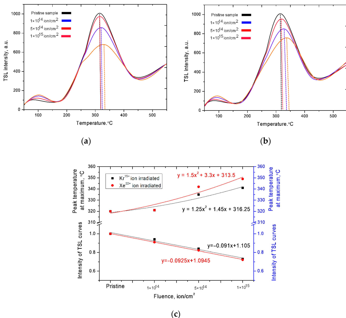
Figure 1. Thermally stimulated luminescence (TSL) curves of the studied ceramics depending on the heating temperature: (a) Kr 15+ ion irradiated dose; (b) Xe 22+ ion irradiated dose; (c) Graph of changes in the TSL curves' intensity and maximum temperature depending on the irradiation fluence.
