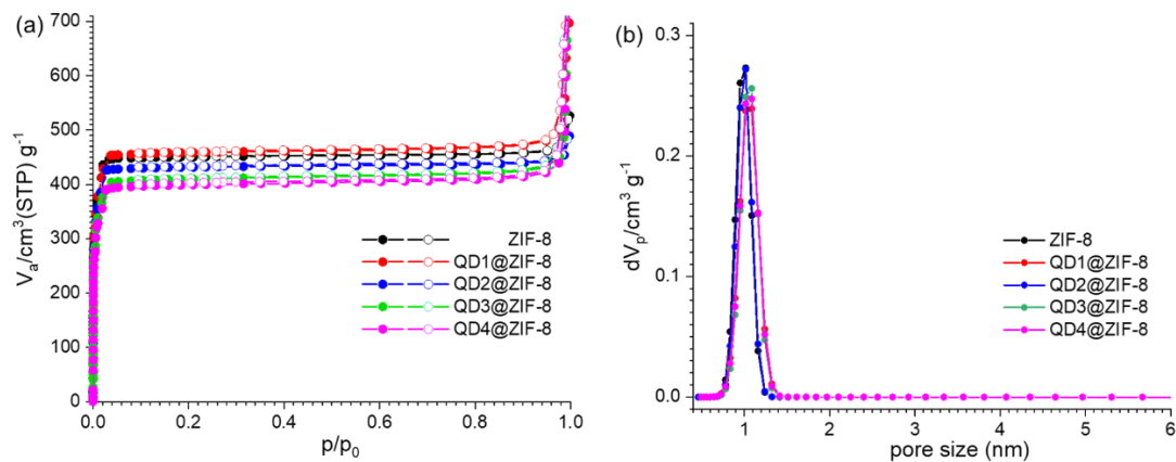
Figure S1. (a) Nitrogen adsorption (solid) and desorption (cycle) curves and (b) pore size distribution of CdS QDs@ZIF-8 samples.
