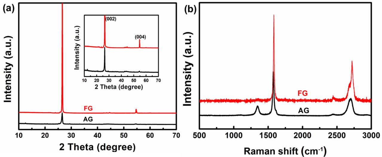
Figure S1. (a) XRD patterns and (b) Raman spectra of AG and FG.
