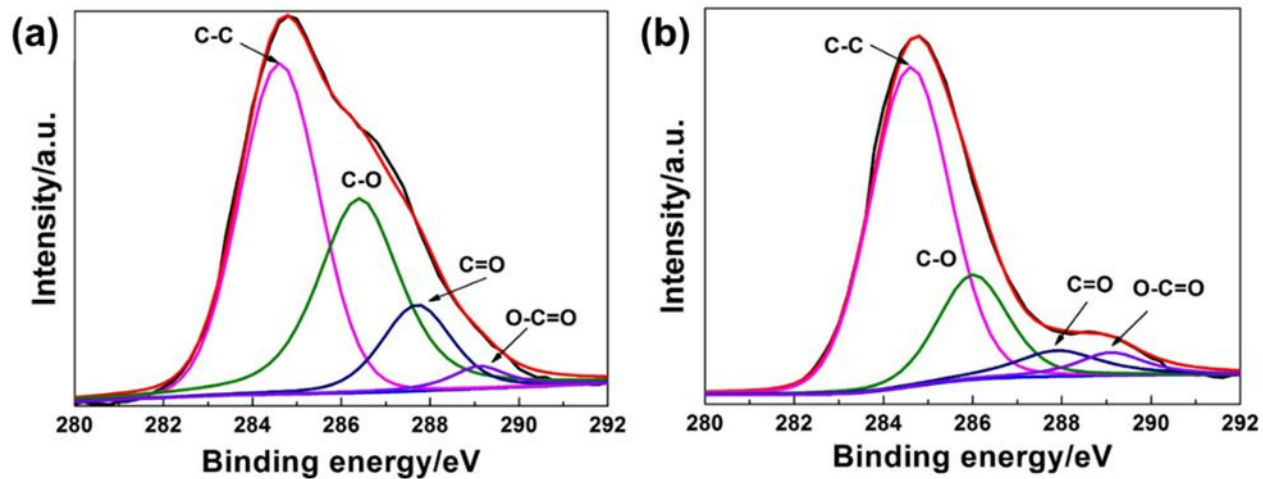
Figure S2. XPS patterns of GO-QDs (a) and GQDs (b).
