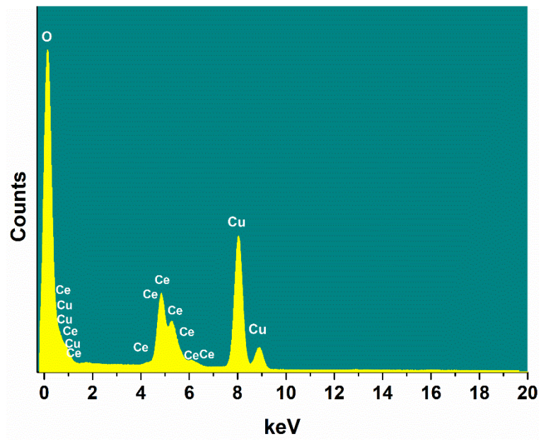
Figure S3. EDX spectra of CeO 2 NP.
