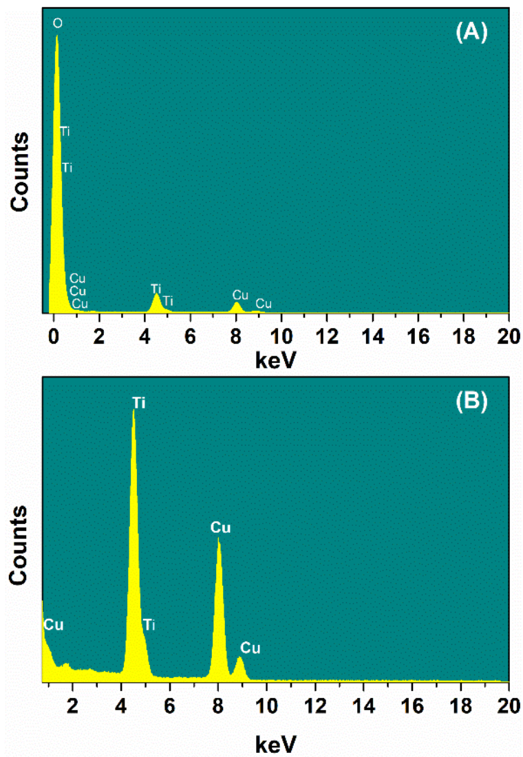
Figure S1. EDX spectra of TiO 2 NP from 0 to 20 keV (A) and from 1 to 20 keV (B).
