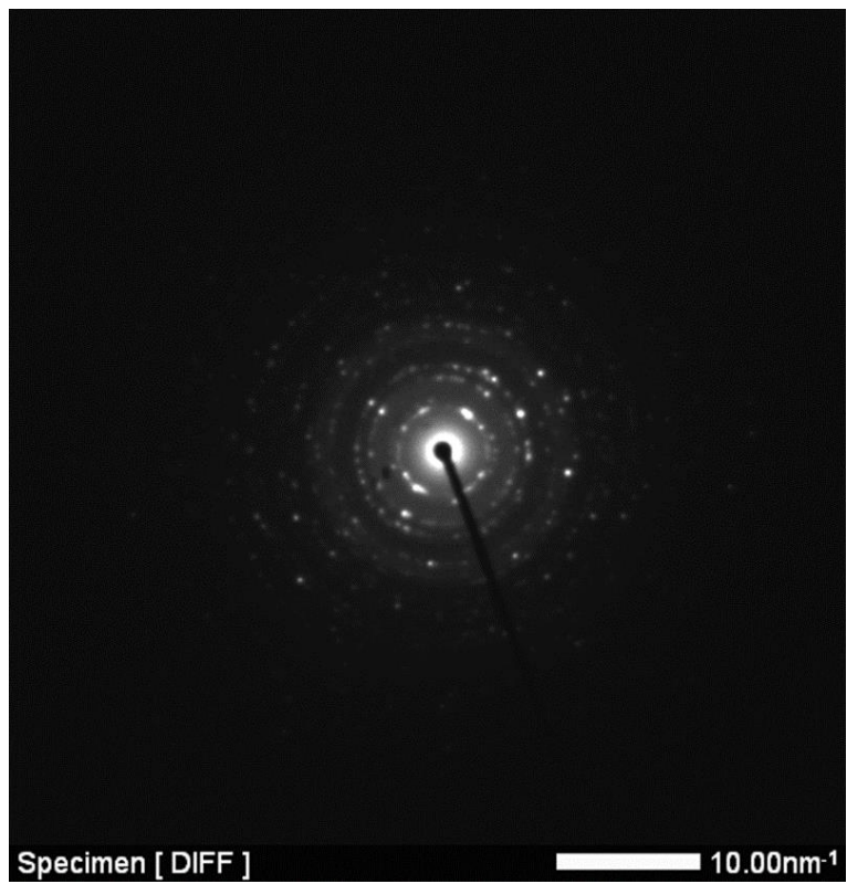
Figure S4. SAED pattern of CeO 2 NP.
